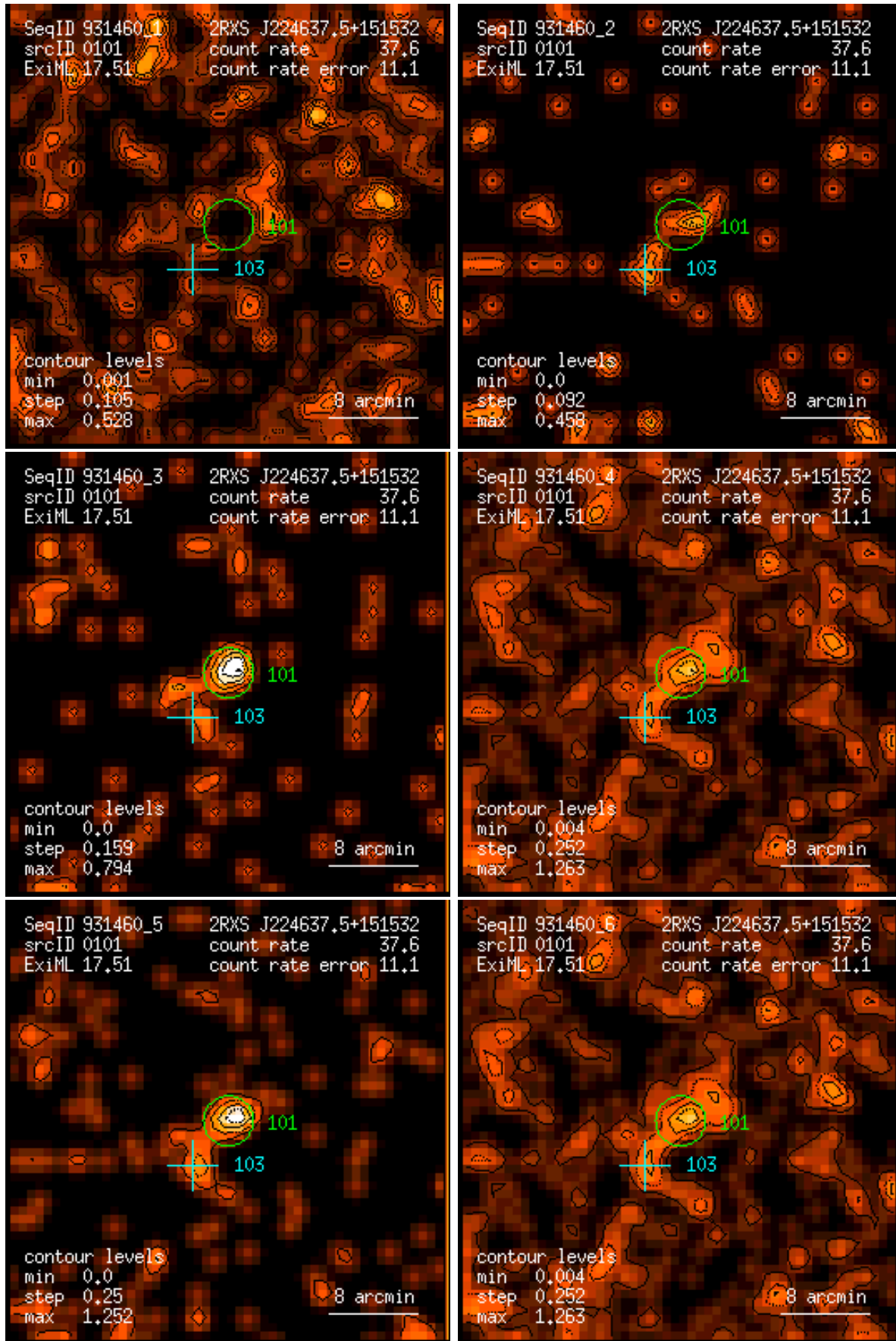
Figure 101: RASS 931460: detection 0101: band rate images, Gaussian filter: (1) PSPC channels 11 – 41, (2) 52 – 90, (3) 91 – 201, (4) 11 – 235, (5) 52 – 201, (6) 11 – 201. Broad band rates in counts/ks. Band rate contour levels in counts/ks/arcmin 2 .
