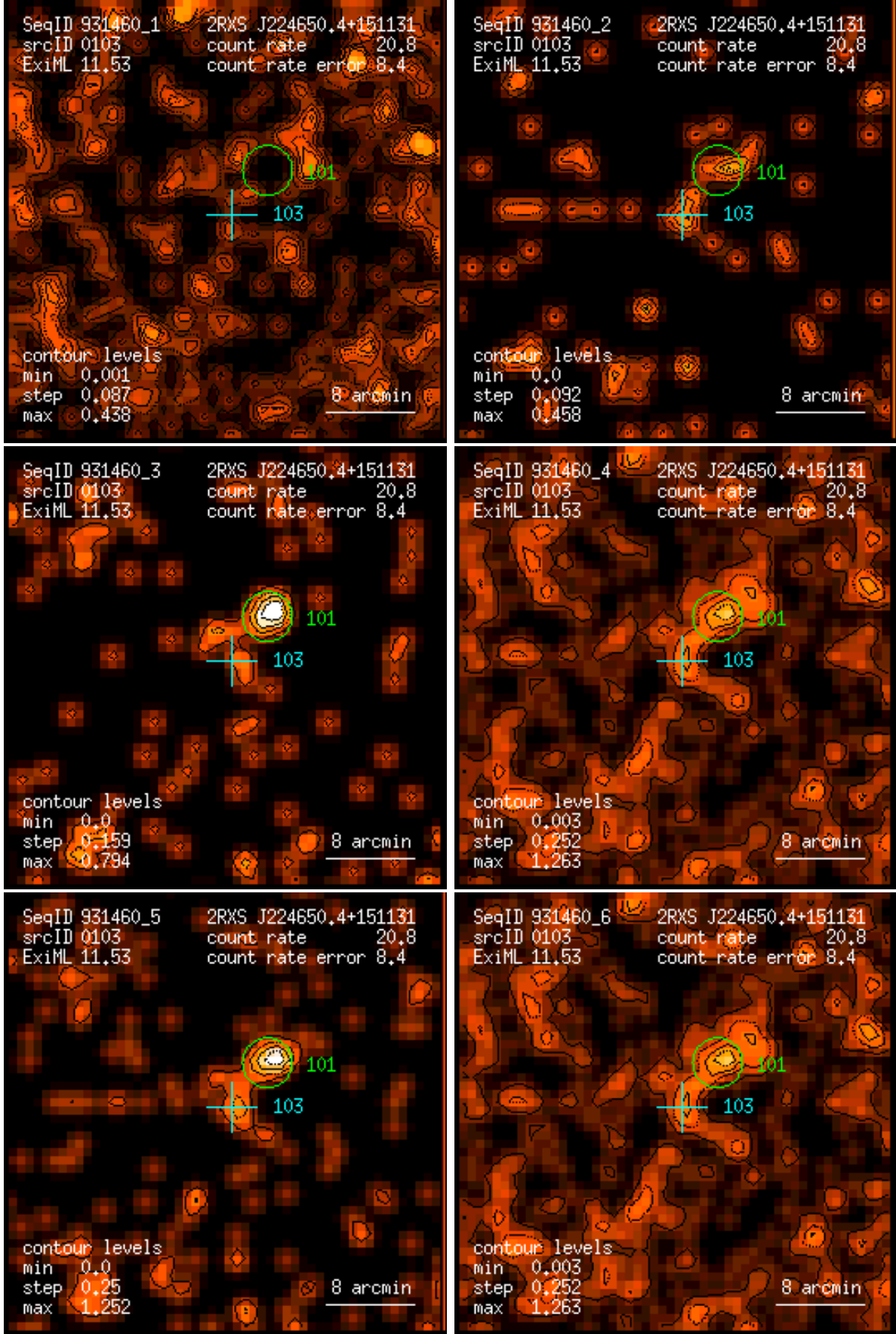
Figure 103: RASS 931460: detection 0103: band rate images, Gaussian filter: (1) PSPC channels 11 – 41, (2) 52 – 90, (3) 91 – 201, (4) 11 – 235, (5) 52 – 201, (6) 11 – 201. Broad band rates in counts/ks. Band rate contour levels in counts/ks/arcmin 2 .
