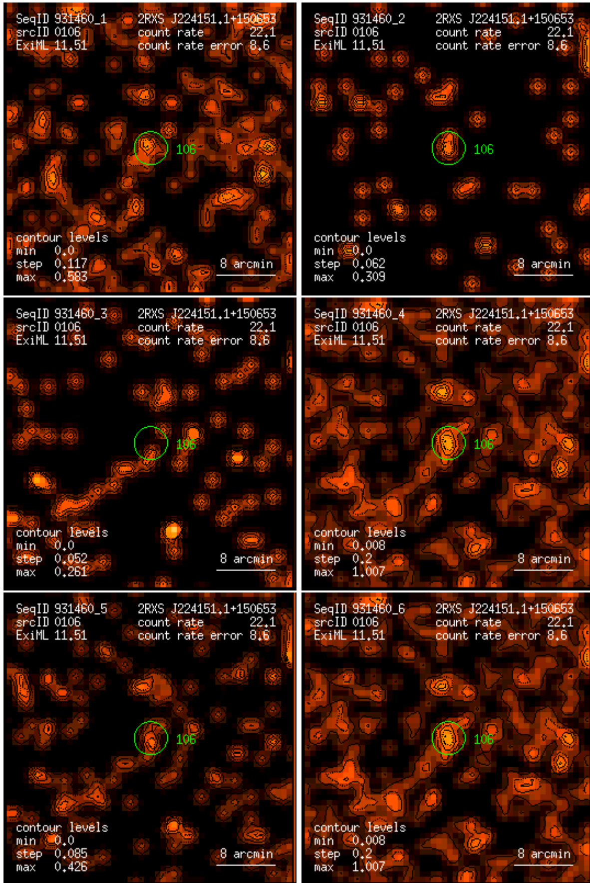
Figure 106: RASS 931460: detection 0106: band rate images, Gaussian filter: (1) PSPC channels 11 – 41, (2) 52 – 90, (3) 91 – 201, (4) 11 – 235, (5) 52 – 201, (6) 11 – 201. Broad band rates in counts/ks. Band rate contour levels in counts/ks/arcmin 2 .
