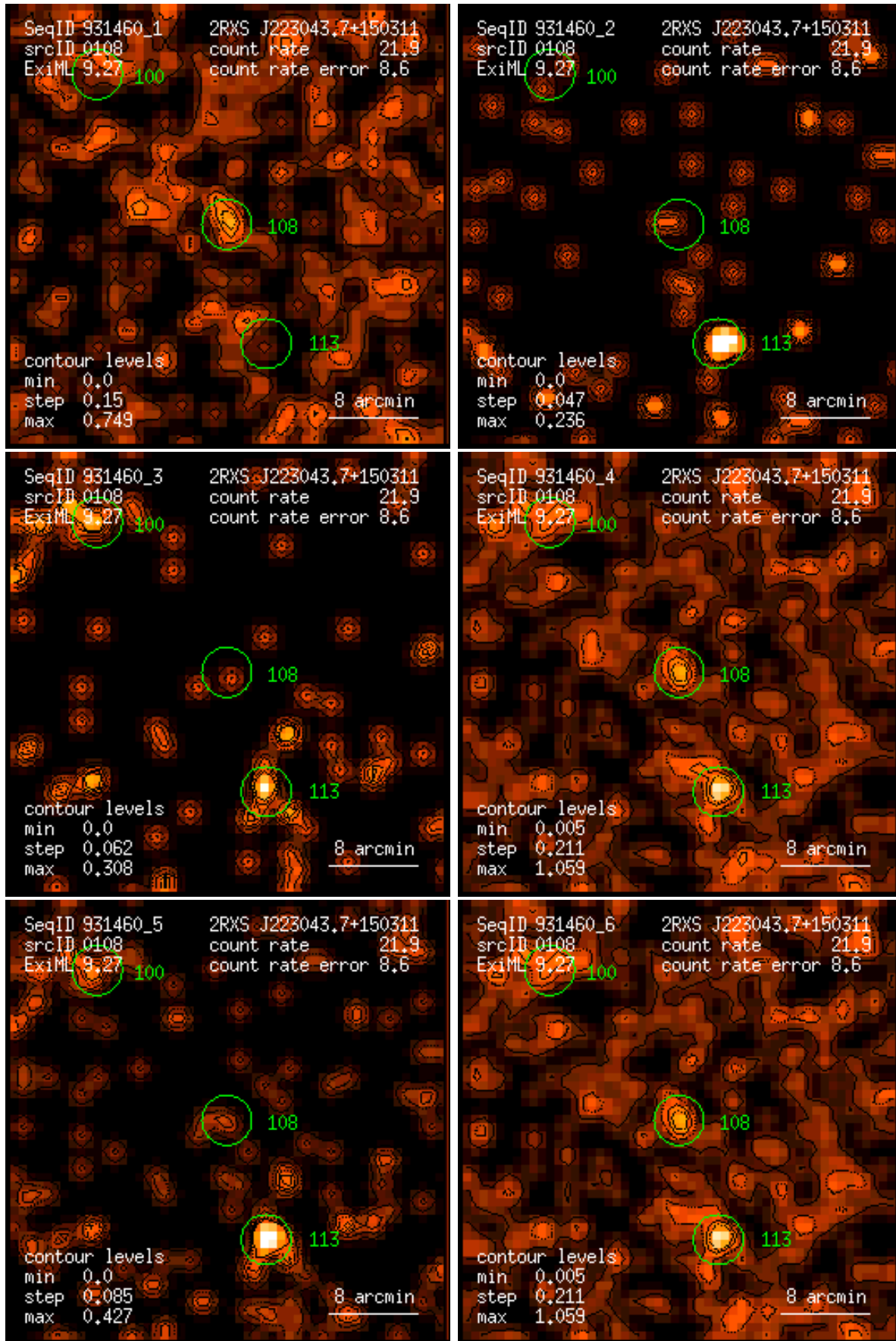
Figure 108: RASS 931460: detection 0108: band rate images, Gaussian filter: (1) PSPC channels 11 – 41, (2) 52 – 90, (3) 91 – 201, (4) 11 – 235, (5) 52 – 201, (6) 11 – 201. Broad band rates in counts/ks. Band rate contour levels in counts/ks/arcmin 2 .
