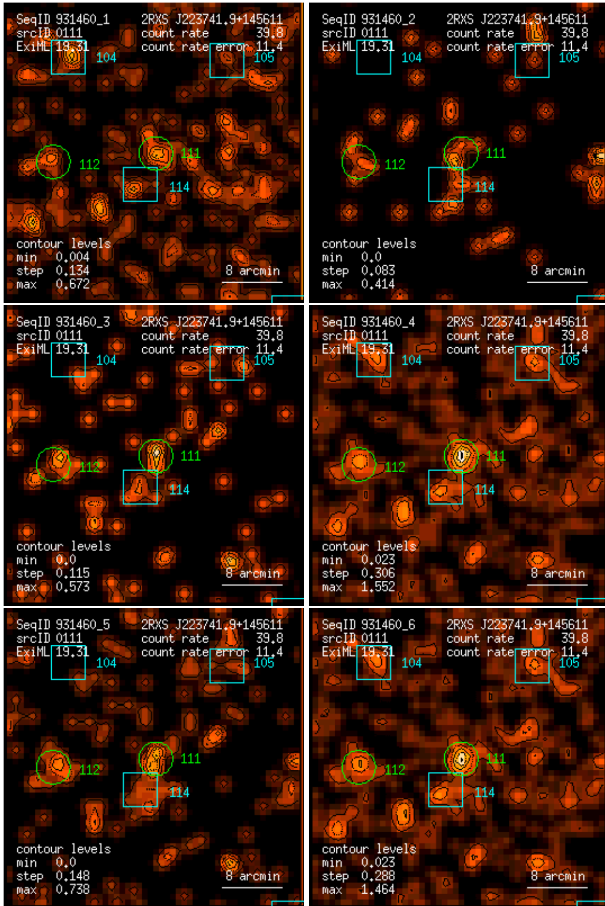
Figure 111: RASS 931460: detection 0111: band rate images, Gaussian filter: (1) PSPC channels 11 – 41, (2) 52 – 90, (3) 91 – 201, (4) 11 – 235, (5) 52 – 201, (6) 11 – 201. Broad band rates in counts/ks. Band rate contour levels in counts/ks/arcmin 2 .
