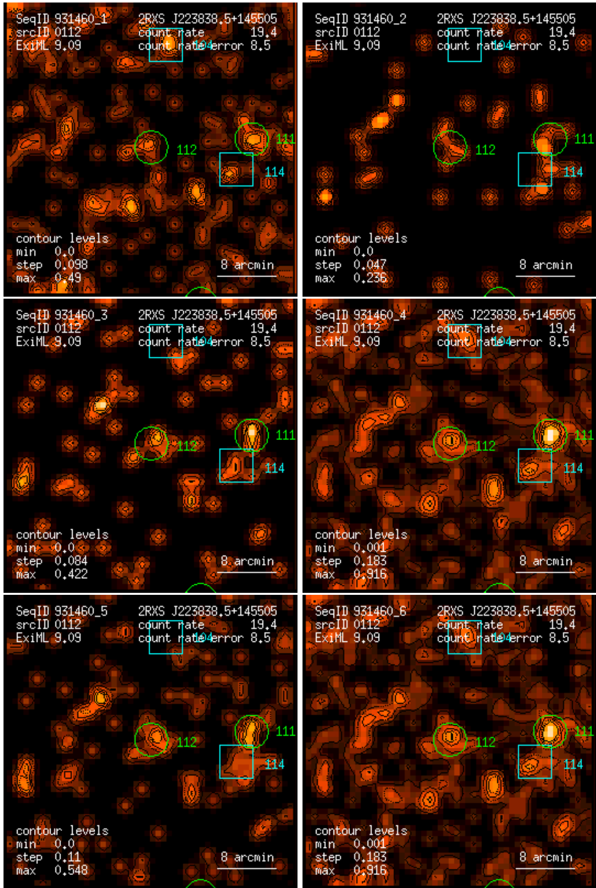
Figure 112: RASS 931460: detection 0112: band rate images, Gaussian filter: (1) PSPC channels 11 – 41, (2) 52 – 90, (3) 91 – 201, (4) 11 – 235, (5) 52 – 201, (6) 11 – 201. Broad band rates in counts/ks. Band rate contour levels in counts/ks/arcmin 2 .
