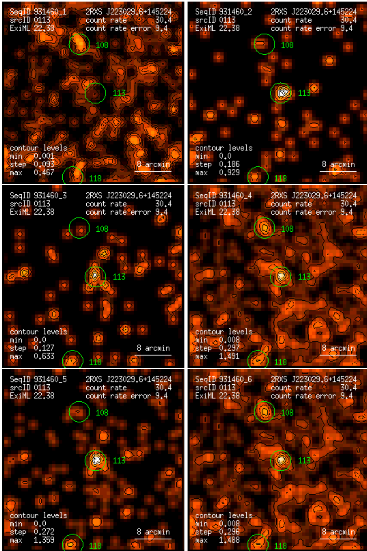
Figure 113: RASS 931460: detection 0113: band rate images, Gaussian filter: (1) PSPC channels 11 – 41, (2) 52 – 90, (3) 91 – 201, (4) 11 – 235, (5) 52 – 201, (6) 11 – 201. Broad band rates in counts/ks. Band rate contour levels in counts/ks/arcmin 2 .
