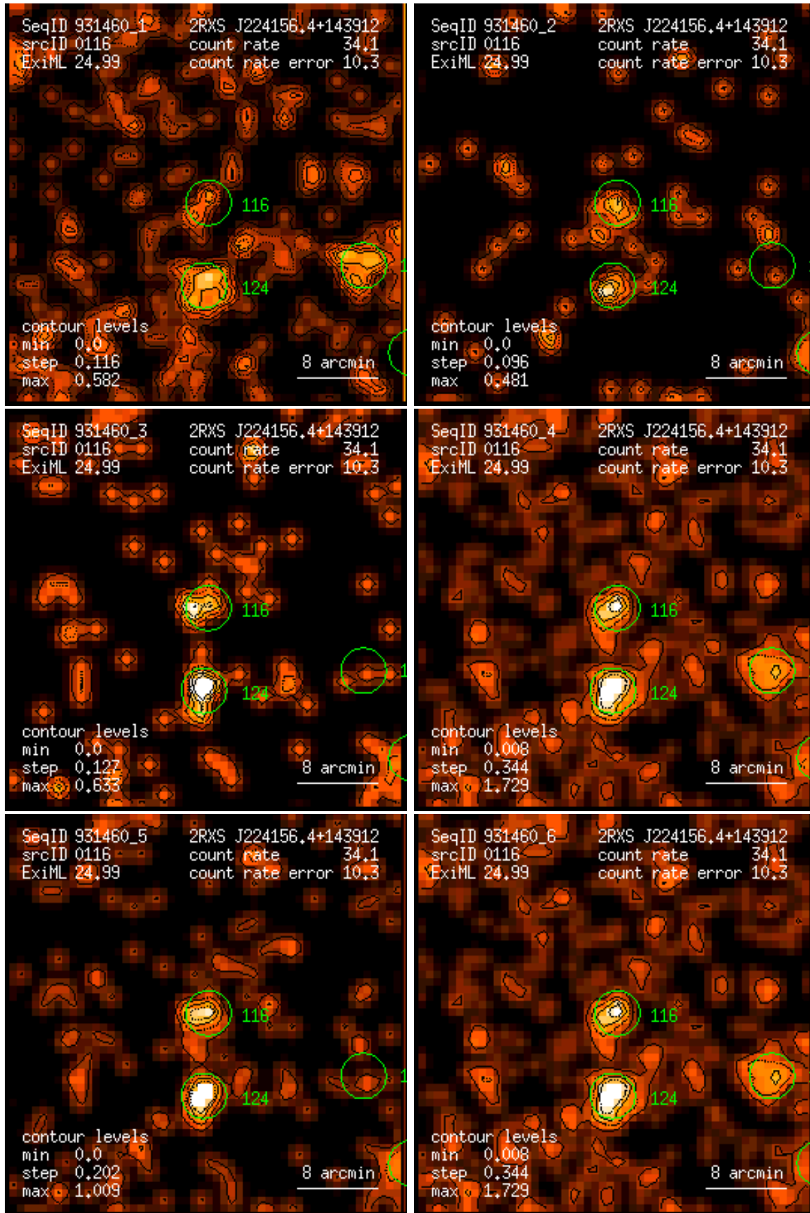
Figure 116: RASS 931460: detection 0116: band rate images, Gaussian filter: (1) PSPC channels 11 – 41, (2) 52 – 90, (3) 91 – 201, (4) 11 – 235, (5) 52 – 201, (6) 11 – 201. Broad band rates in counts/ks. Band rate contour levels in counts/ks/arcmin 2 .
