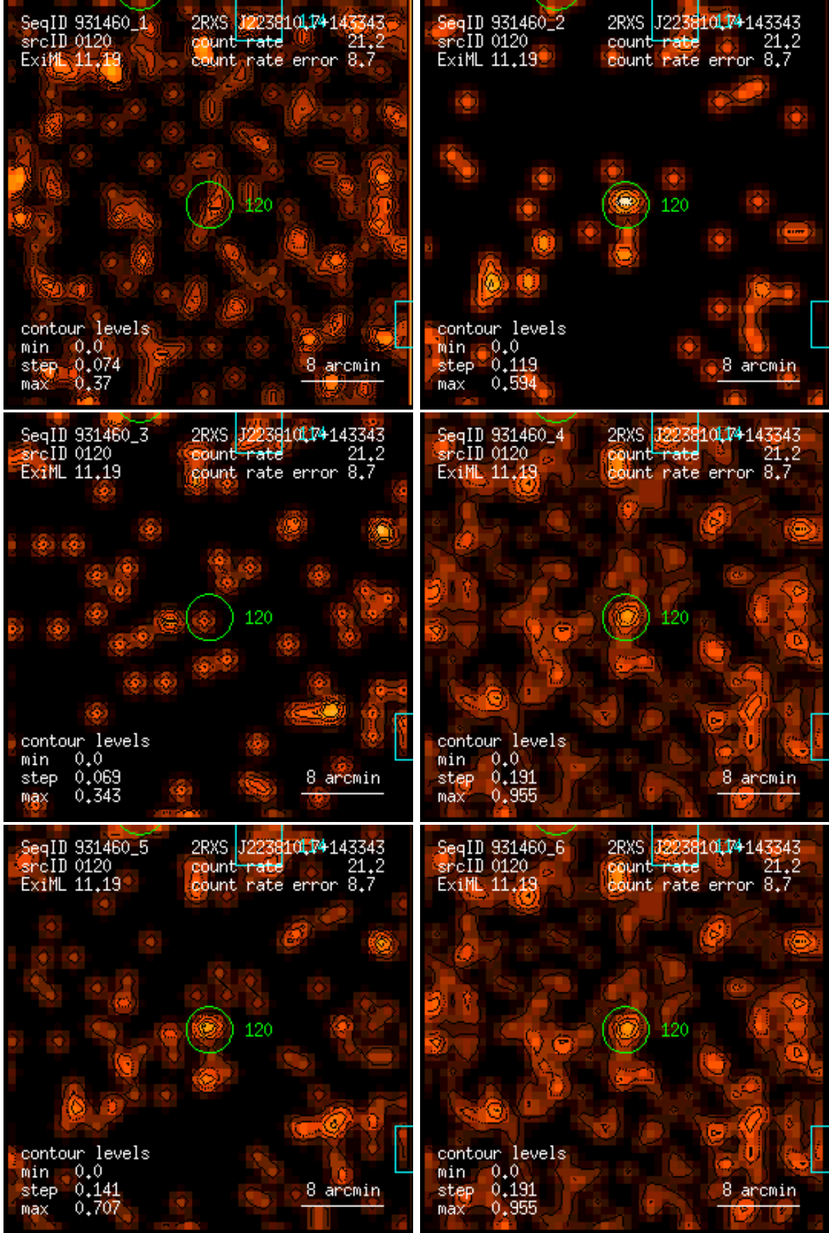
Figure 120: RASS 931460: detection 0120: band rate images, Gaussian filter: (1) PSPC channels 11 – 41, (2) 52 – 90, (3) 91 – 201, (4) 11 – 235, (5) 52 – 201, (6) 11 – 201. Broad band rates in counts/ks. Band rate contour levels in counts/ks/arcmin 2 .
