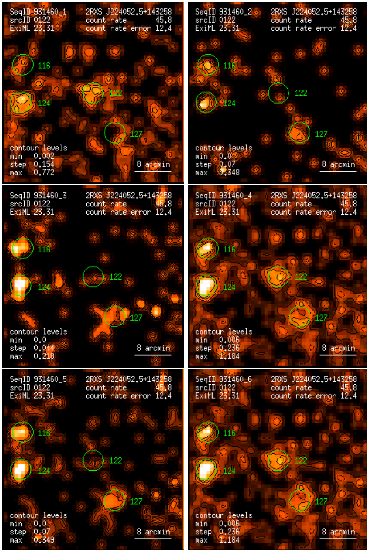
Figure 122: RASS 931460: detection 0122: band rate images, Gaussian filter: (1) PSPC channels 11 – 41, (2) 52 – 90, (3) 91 – 201, (4) 11 – 235, (5) 52 – 201, (6) 11 – 201. Broad band rates in counts/ks. Band rate contour levels in counts/ks/arcmin 2 .
