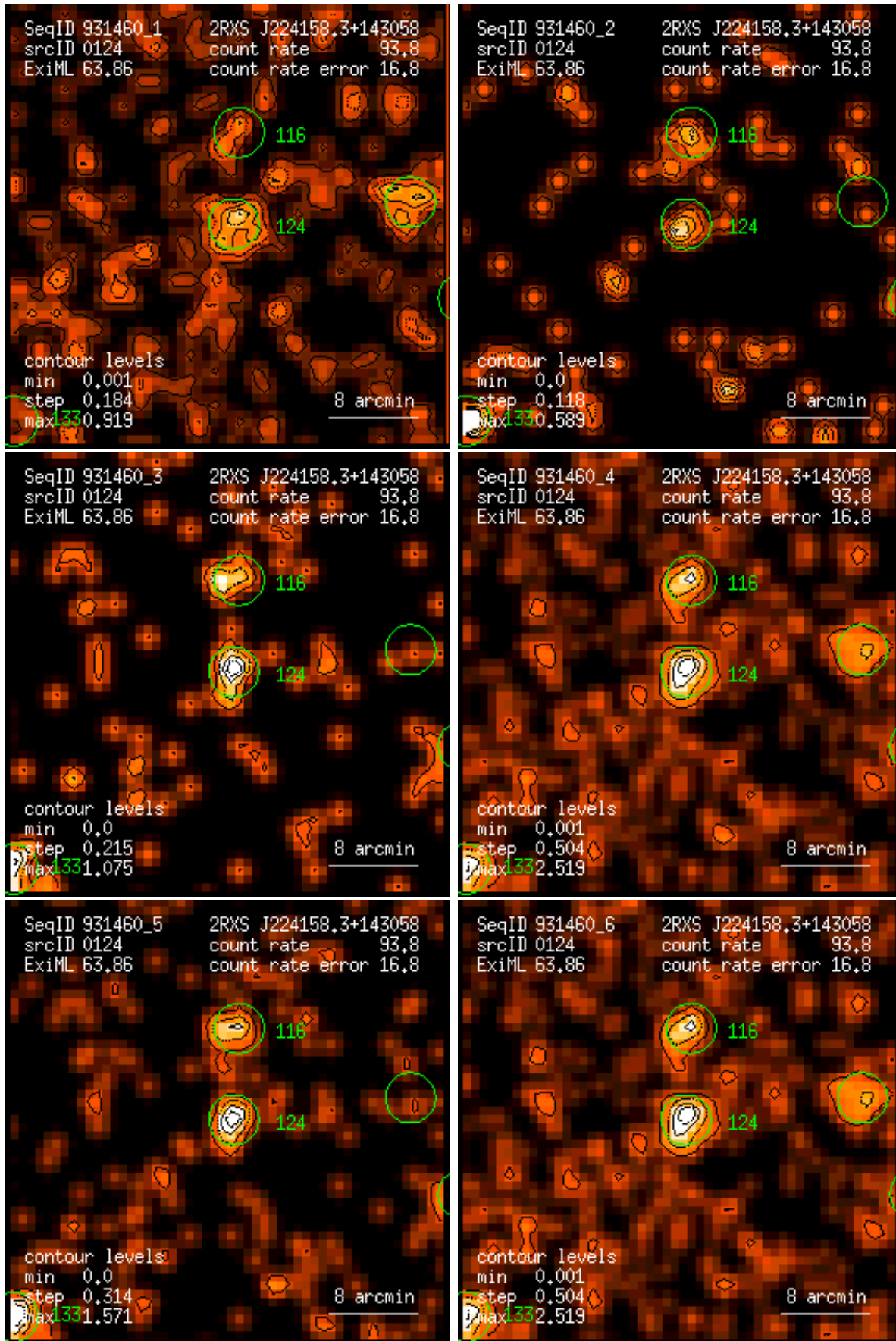
Figure 124: RASS 931460: detection 0124: band rate images, Gaussian filter: (1) PSPC channels 11 – 41, (2) 52 – 90, (3) 91 – 201, (4) 11 – 235, (5) 52 – 201, (6) 11 – 201. Broad band rates in counts/ks. Band rate contour levels in counts/ks/arcmin 2 .
