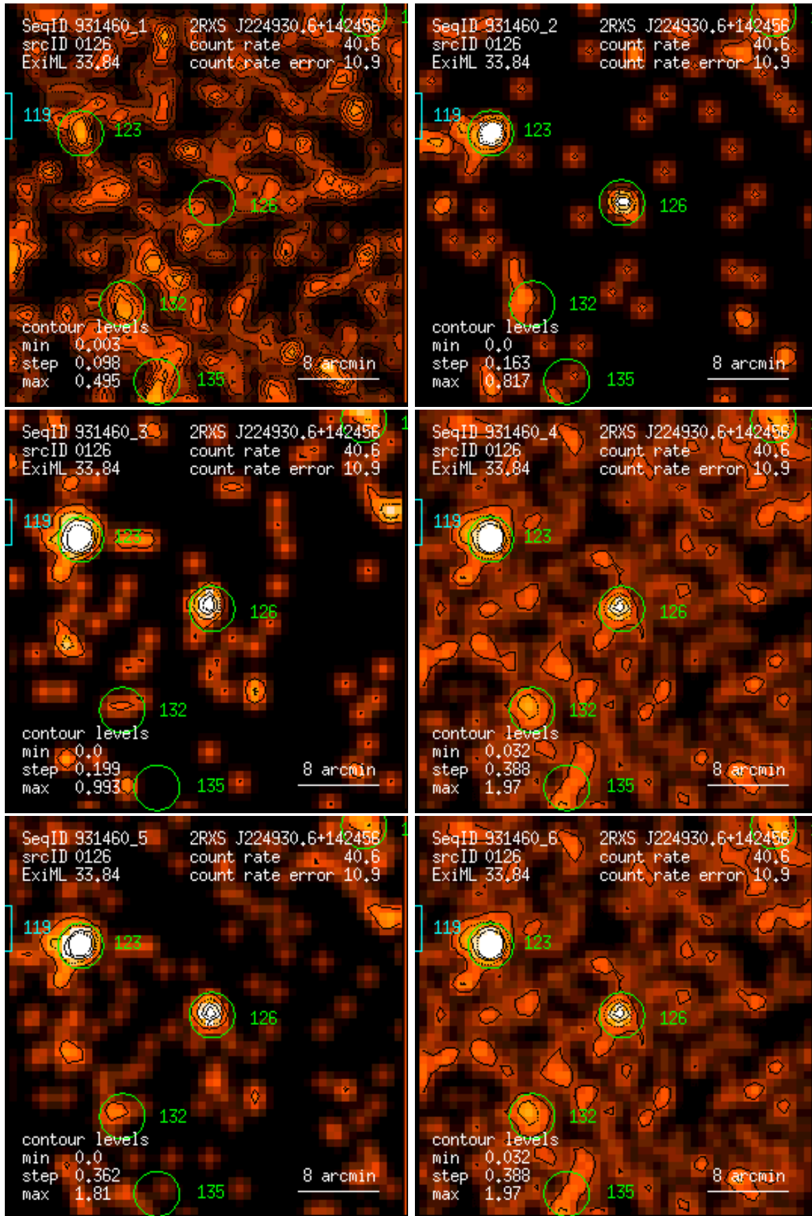
Figure 126: RASS 931460: detection 0126: band rate images, Gaussian filter: (1) PSPC channels 11 – 41, (2) 52 – 90, (3) 91 – 201, (4) 11 – 235, (5) 52 – 201, (6) 11 – 201. Broad band rates in counts/ks. Band rate contour levels in counts/ks/arcmin 2 .
