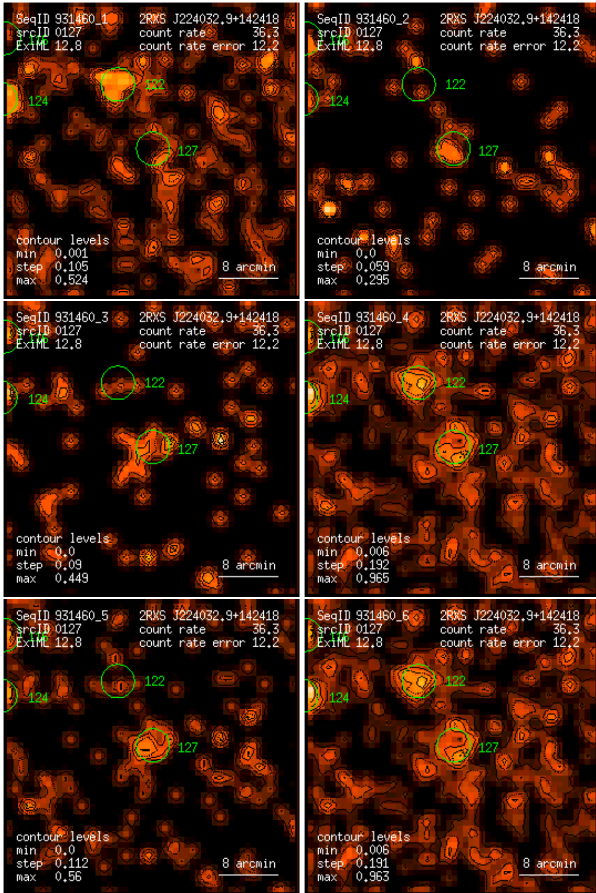
Figure 127: RASS 931460: detection 0127: band rate images, Gaussian filter: (1) PSPC channels 11 – 41, (2) 52 – 90, (3) 91 – 201, (4) 11 – 235, (5) 52 – 201, (6) 11 – 201. Broad band rates in counts/ks. Band rate contour levels in counts/ks/arcmin 2 .
