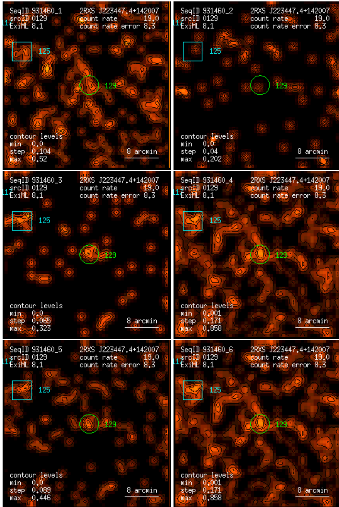
Figure 129: RASS 931460: detection 0129: band rate images, Gaussian filter: (1) PSPC channels 11 – 41, (2) 52 – 90, (3) 91 – 201, (4) 11 – 235, (5) 52 – 201, (6) 11 – 201. Broad band rates in counts/ks. Band rate contour levels in counts/ks/arcmin 2 .
