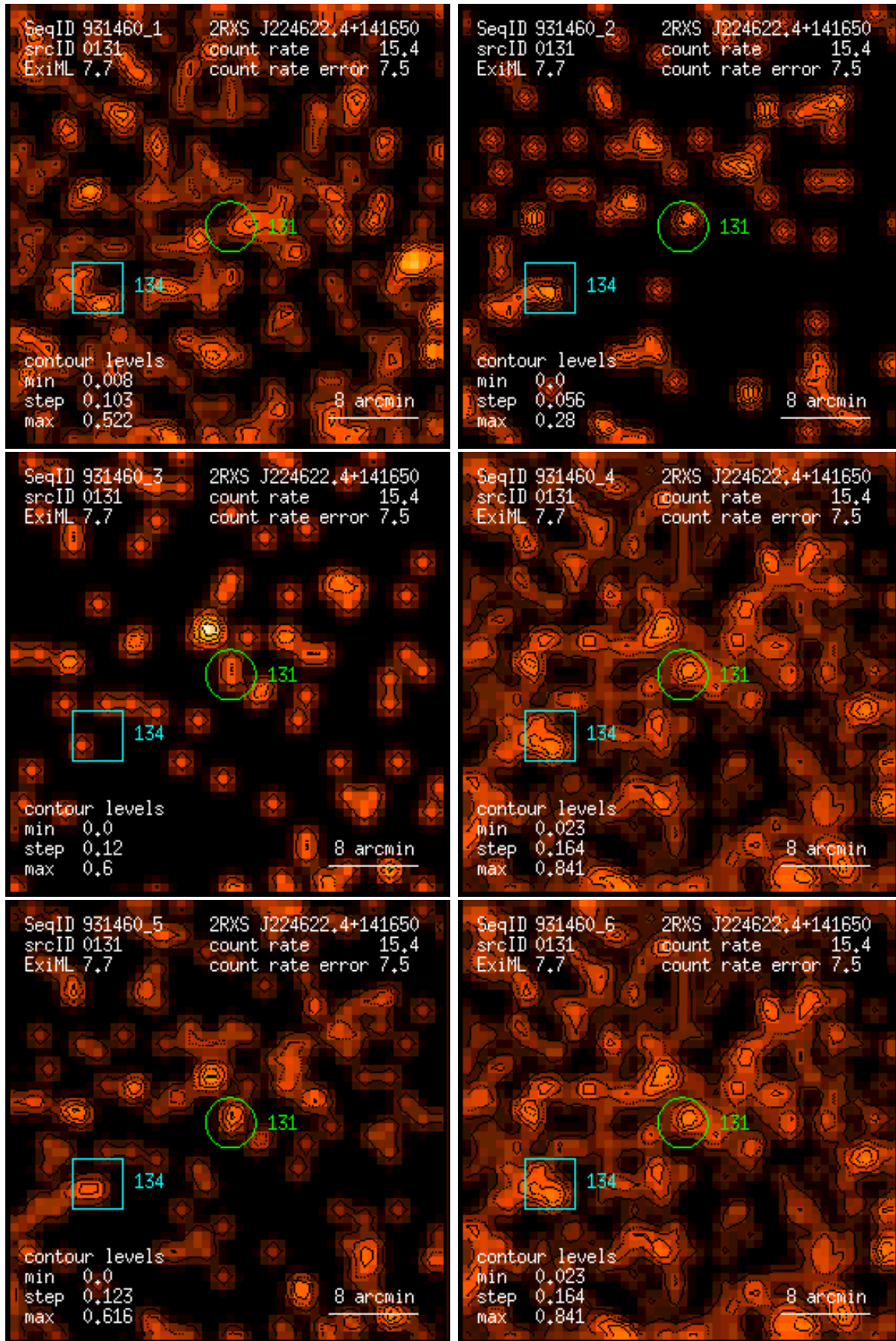
Figure 131: RASS 931460: detection 0131: band rate images, Gaussian filter: (1) PSPC channels 11 – 41, (2) 52 – 90, (3) 91 – 201, (4) 11 – 235, (5) 52 – 201, (6) 11 – 201. Broad band rates in counts/ks. Band rate contour levels in counts/ks/arcmin 2 .
