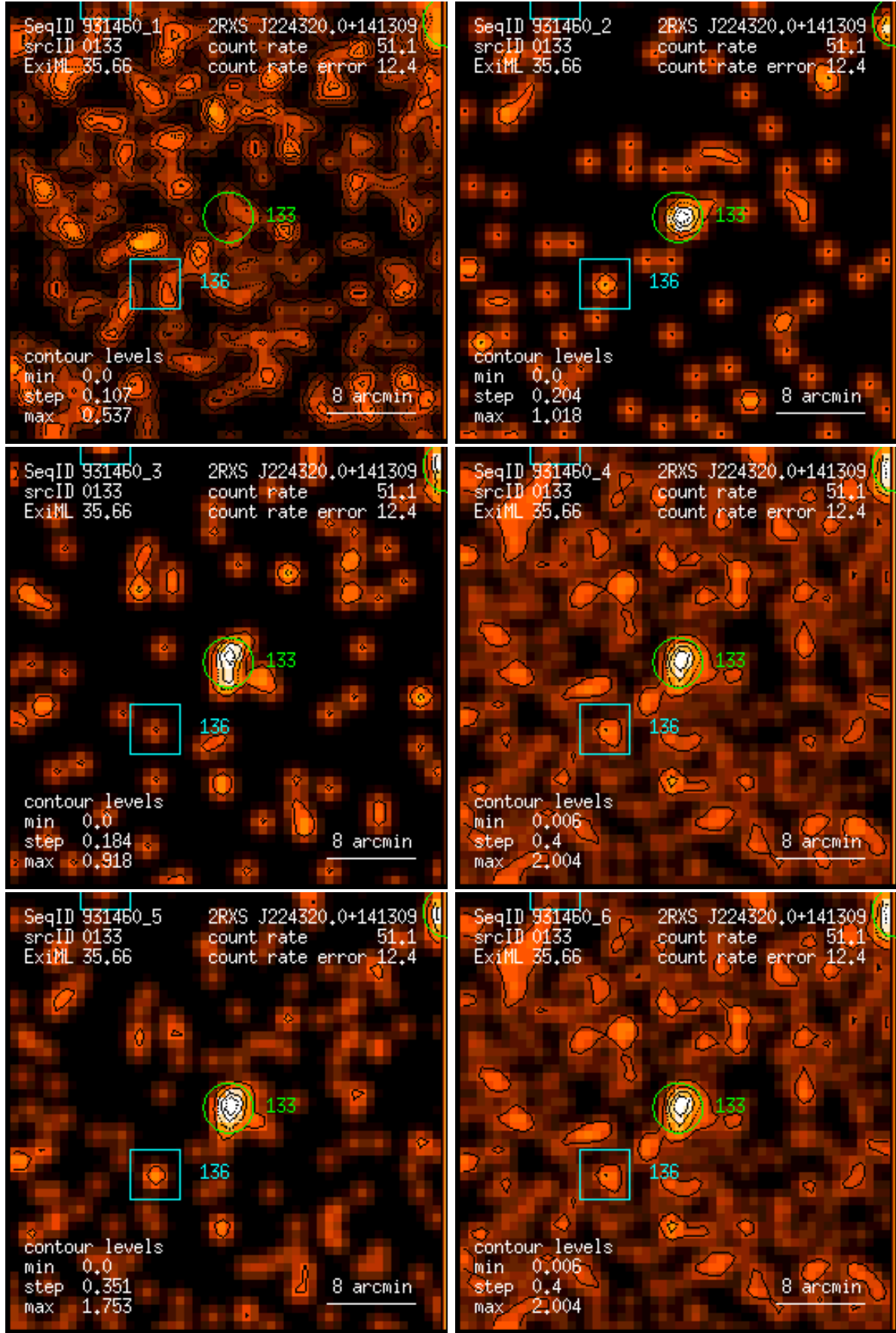
Figure 133: RASS 931460: detection 0133: band rate images, Gaussian filter: (1) PSPC channels 11 – 41, (2) 52 – 90, (3) 91 – 201, (4) 11 – 235, (5) 52 – 201, (6) 11 – 201. Broad band rates in counts/ks. Band rate contour levels in counts/ks/arcmin 2 .
