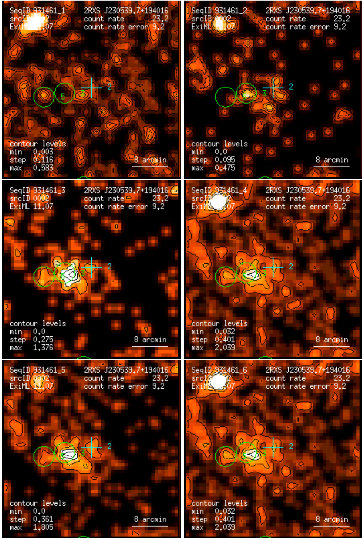
Figure 2: RASS 931461: detection 0002: band rate images, Gaussian filter: (1) PSPC channels 11 – 41, (2) 52 – 90, (3) 91 – 201, (4) 11 – 235, (5) 52 – 201, (6) 11 – 201. Broad band rates in counts/ks. Band rate contour levels in counts/ks/arcmin 2 .
