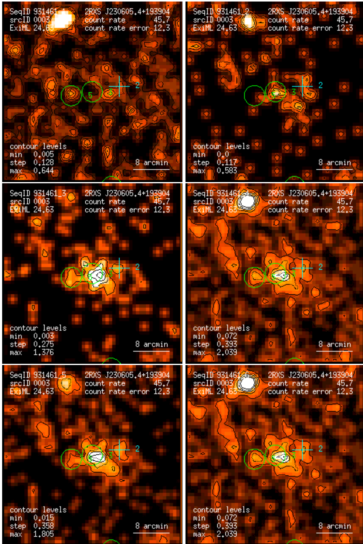
Figure 3: RASS 931461: detection 0003: band rate images, Gaussian filter: (1) PSPC channels 11 – 41, (2) 52 – 90, (3) 91 – 201, (4) 11 – 235, (5) 52 – 201, (6) 11 – 201. Broad band rates in counts/ks. Band rate contour levels in counts/ks/arcmin 2 .
