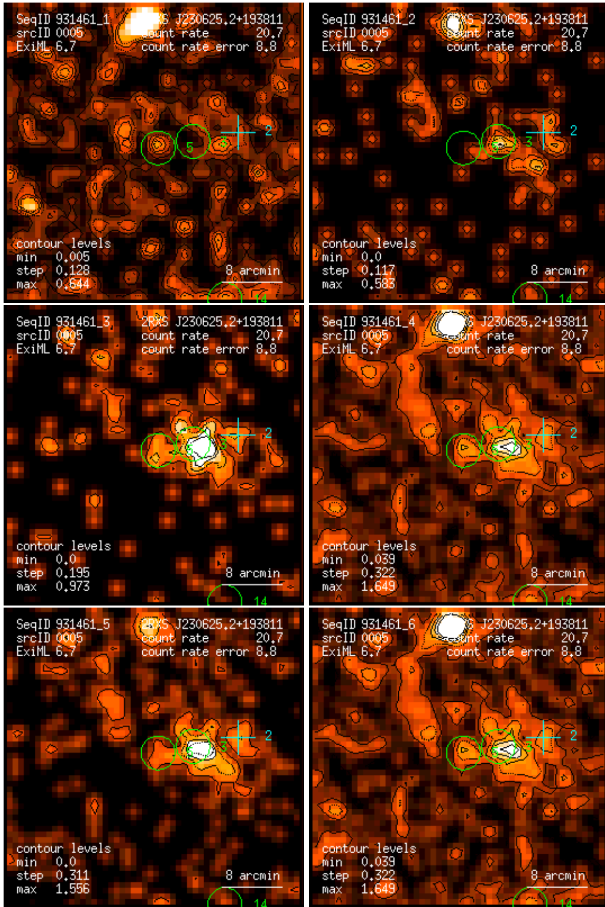
Figure 5: RASS 931461: detection 0005: band rate images, Gaussian filter: (1) PSPC channels 11 – 41, (2) 52 – 90, (3) 91 – 201, (4) 11 – 235, (5) 52 – 201, (6) 11 – 201. Broad band rates in counts/ks. Band rate contour levels in counts/ks/arcmin 2 .
