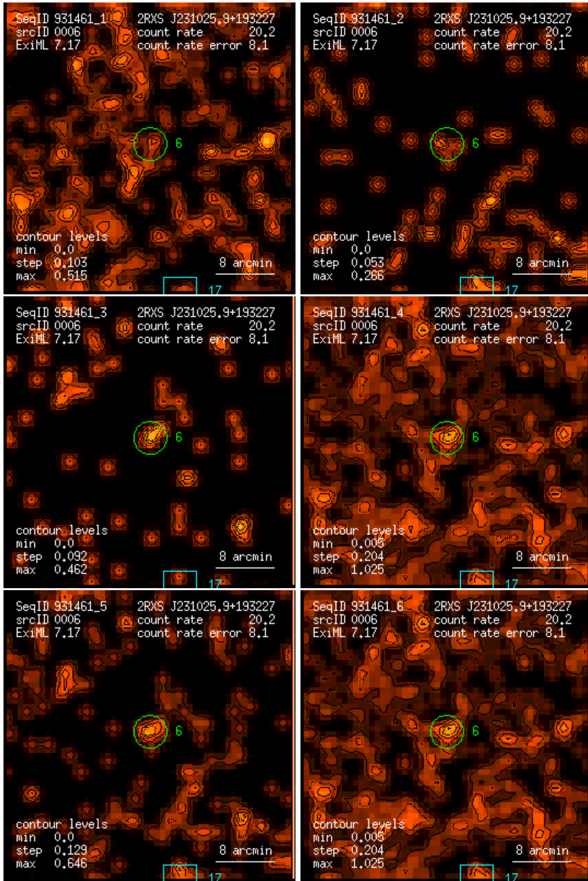
Figure 6: RASS 931461: detection 0006: band rate images, Gaussian filter: (1) PSPC channels 11 – 41, (2) 52 – 90, (3) 91 – 201, (4) 11 – 235, (5) 52 – 201, (6) 11 – 201. Broad band rates in counts/ks. Band rate contour levels in counts/ks/arcmin 2 .
