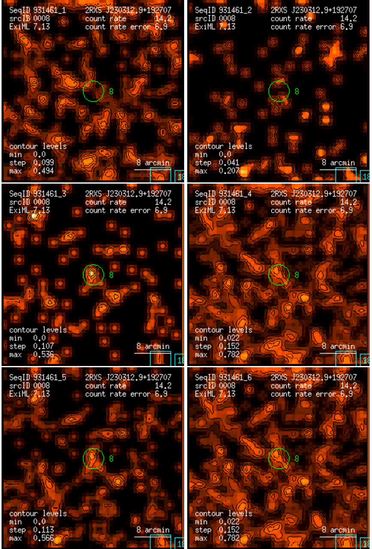
Figure 8: RASS 931461: detection 0008: band rate images, Gaussian filter: (1) PSPC channels 11 – 41, (2) 52 – 90, (3) 91 – 201, (4) 11 – 235, (5) 52 – 201, (6) 11 – 201. Broad band rates in counts/ks. Band rate contour levels in counts/ks/arcmin 2 .
