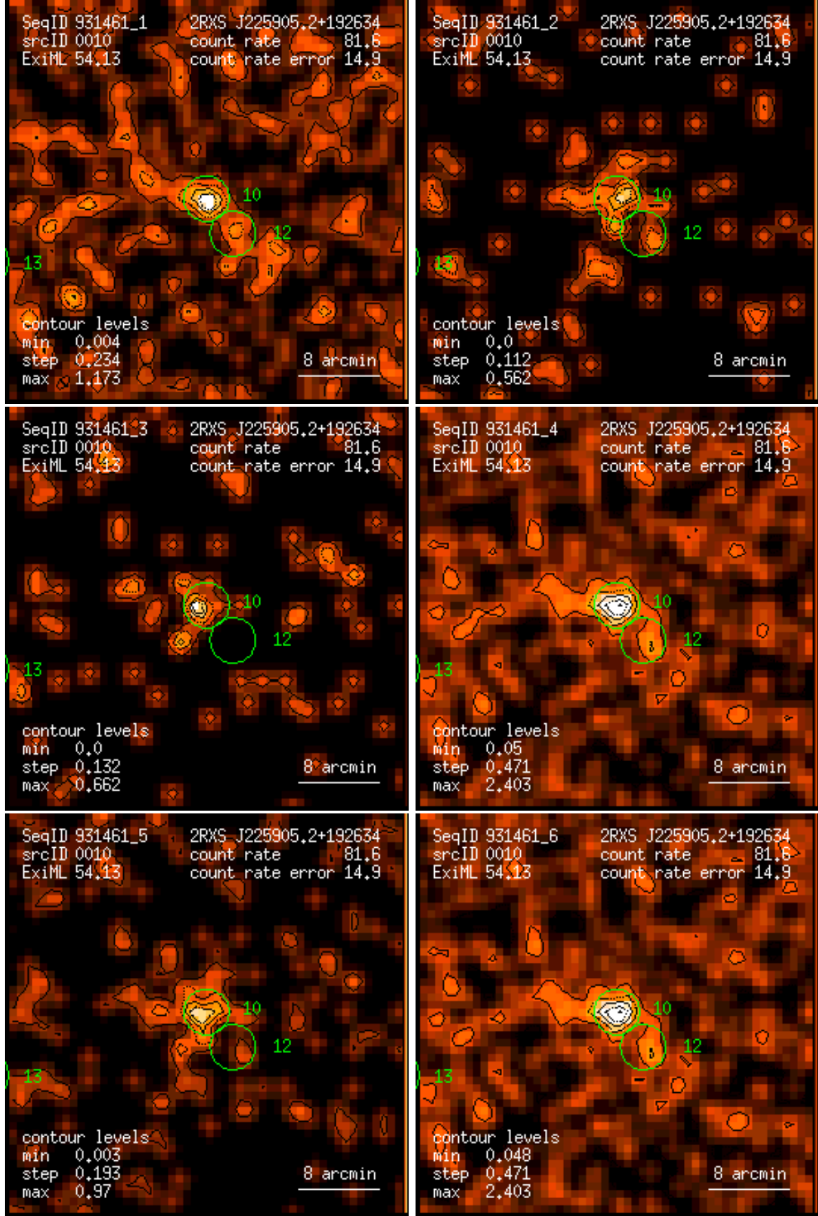
Figure 10: RASS 931461: detection 0010: band rate images, Gaussian filter: (1) PSPC channels 11 – 41, (2) 52 – 90, (3) 91 – 201, (4) 11 – 235, (5) 52 – 201, (6) 11 – 201. Broad band rates in counts/ks. Band rate contour levels in counts/ks/arcmin 2 .
