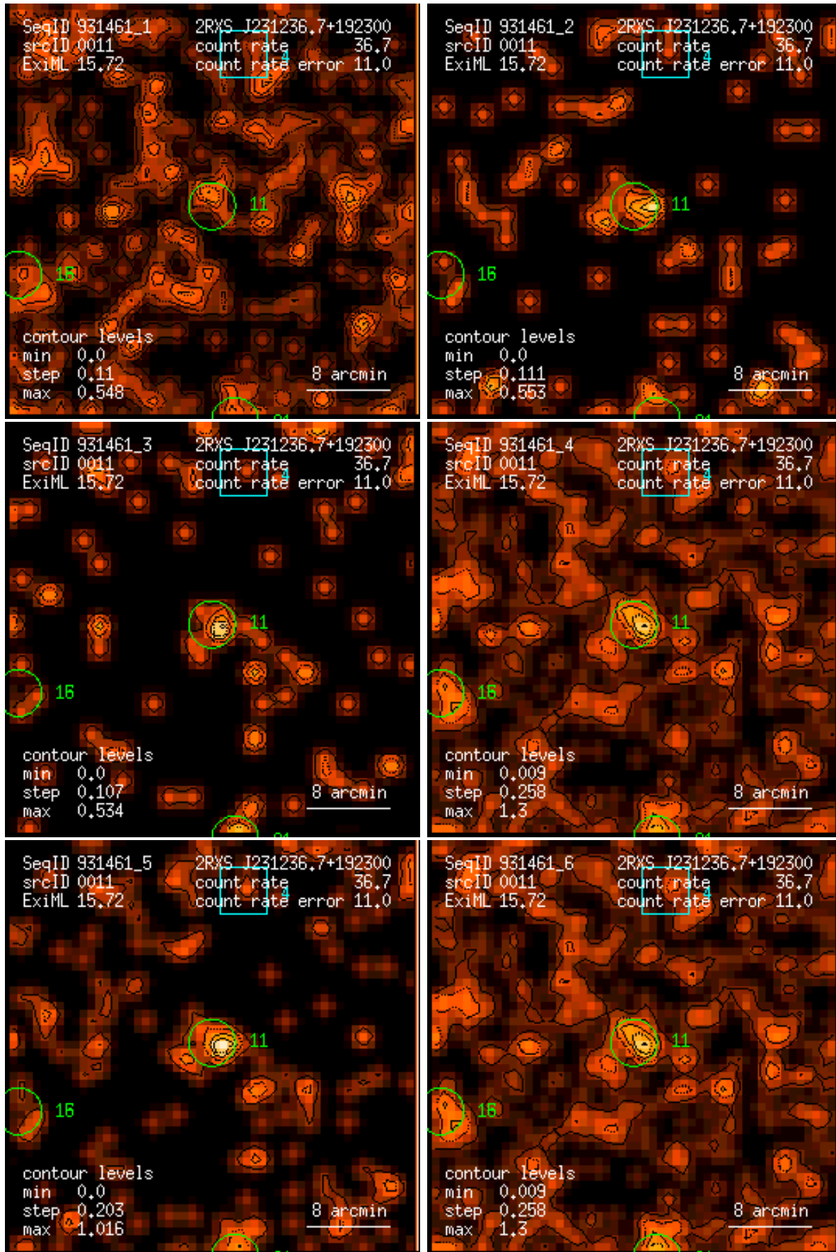
Figure 11: RASS 931461: detection 0011: band rate images, Gaussian filter: (1) PSPC channels 11 – 41, (2) 52 – 90, (3) 91 – 201, (4) 11 – 235, (5) 52 – 201, (6) 11 – 201. Broad band rates in counts/ks. Band rate contour levels in counts/ks/arcmin 2 .
