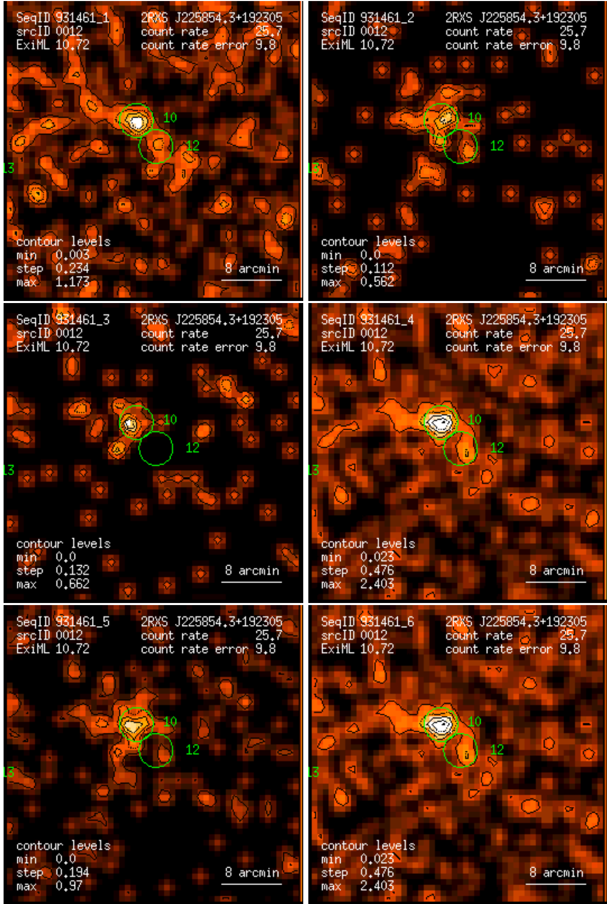
Figure 12: RASS 931461: detection 0012: band rate images, Gaussian filter: (1) PSPC channels 11 – 41, (2) 52 – 90, (3) 91 – 201, (4) 11 – 235, (5) 52 – 201, (6) 11 – 201. Broad band rates in counts/ks. Band rate contour levels in counts/ks/arcmin 2 .
