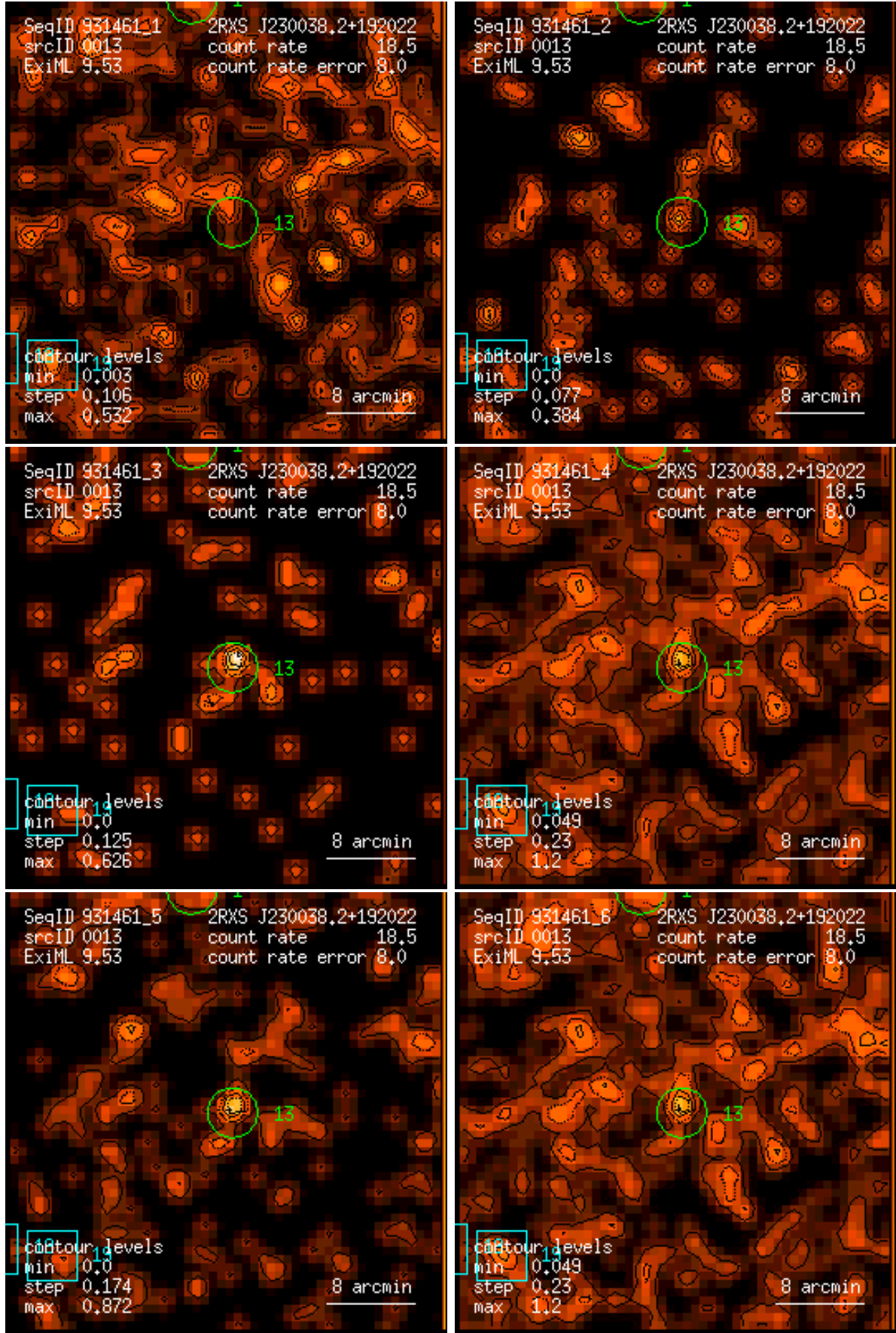
Figure 13: RASS 931461: detection 0013: band rate images, Gaussian filter: (1) PSPC channels 11 – 41, (2) 52 – 90, (3) 91 – 201, (4) 11 – 235, (5) 52 – 201, (6) 11 – 201. Broad band rates in counts/ks. Band rate contour levels in counts/ks/arcmin 2 .
