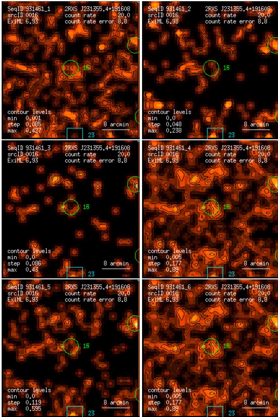
Figure 16: RASS 931461: detection 0016: band rate images, Gaussian filter: (1) PSPC channels 11 – 41, (2) 52 – 90, (3) 91 – 201, (4) 11 – 235, (5) 52 – 201, (6) 11 – 201. Broad band rates in counts/ks. Band rate contour levels in counts/ks/arcmin 2 .
