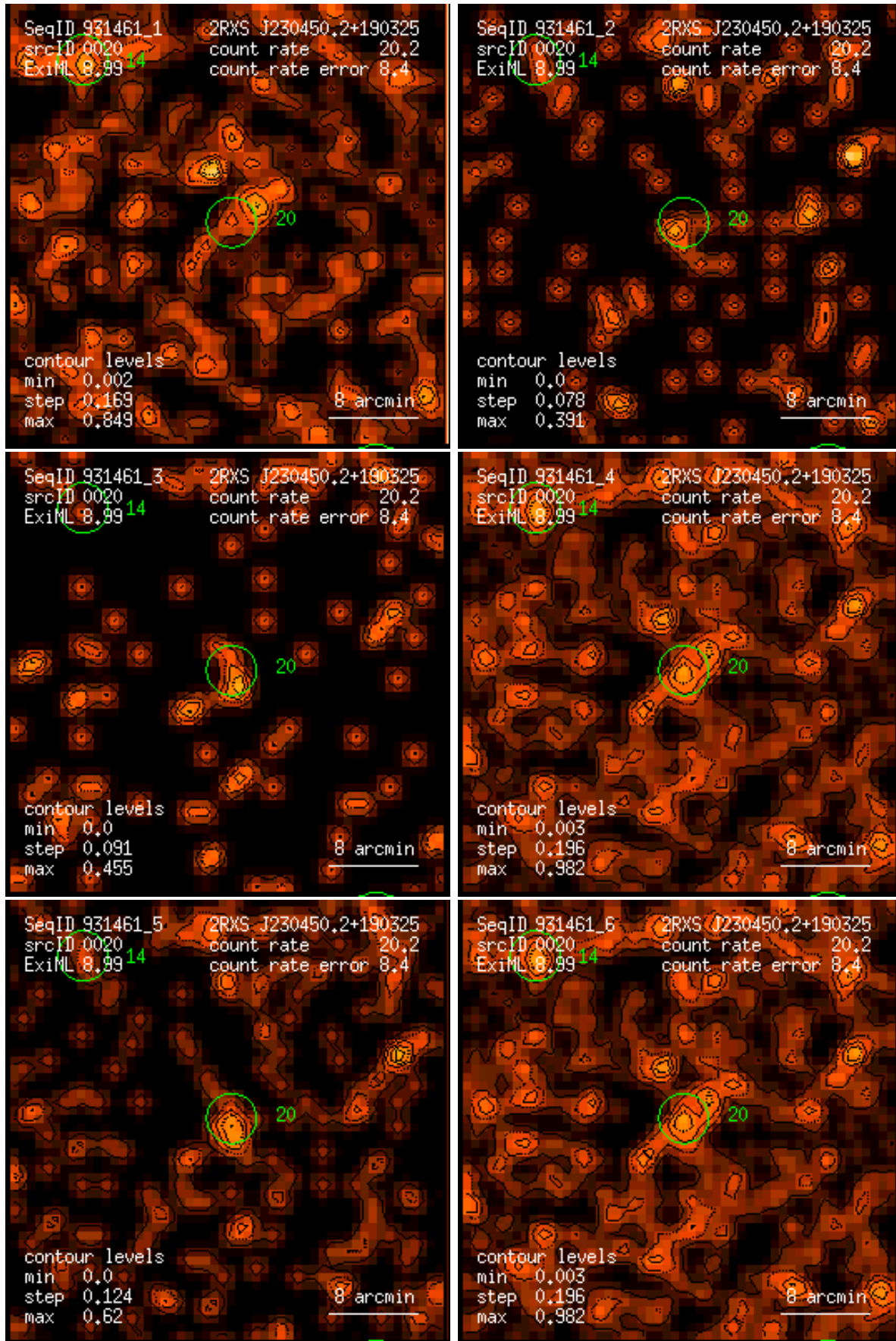
Figure 20: RASS 931461: detection 0020: band rate images, Gaussian filter: (1) PSPC channels 11 – 41, (2) 52 – 90, (3) 91 – 201, (4) 11 – 235, (5) 52 – 201, (6) 11 – 201. Broad band rates in counts/ks. Band rate contour levels in counts/ks/arcmin 2 .
