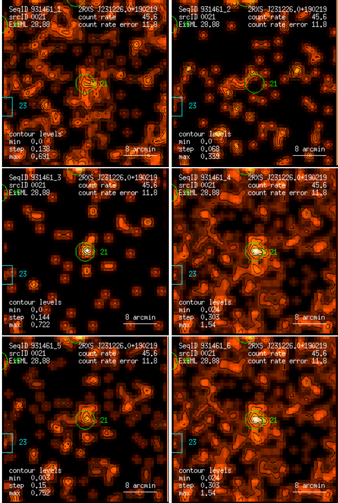
Figure 21: RASS 931461: detection 0021: band rate images, Gaussian filter: (1) PSPC channels 11 – 41, (2) 52 – 90, (3) 91 – 201, (4) 11 – 235, (5) 52 – 201, (6) 11 – 201. Broad band rates in counts/ks. Band rate contour levels in counts/ks/arcmin 2 .
