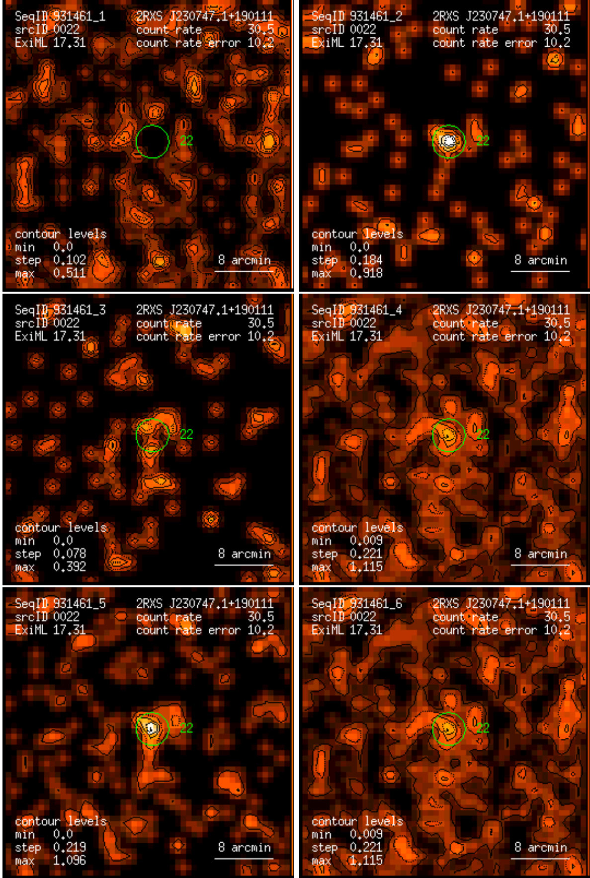
Figure 22: RASS 931461: detection 0022: band rate images, Gaussian filter: (1) PSPC channels 11 – 41, (2) 52 – 90, (3) 91 – 201, (4) 11 – 235, (5) 52 – 201, (6) 11 – 201. Broad band rates in counts/ks. Band rate contour levels in counts/ks/arcmin 2 .
