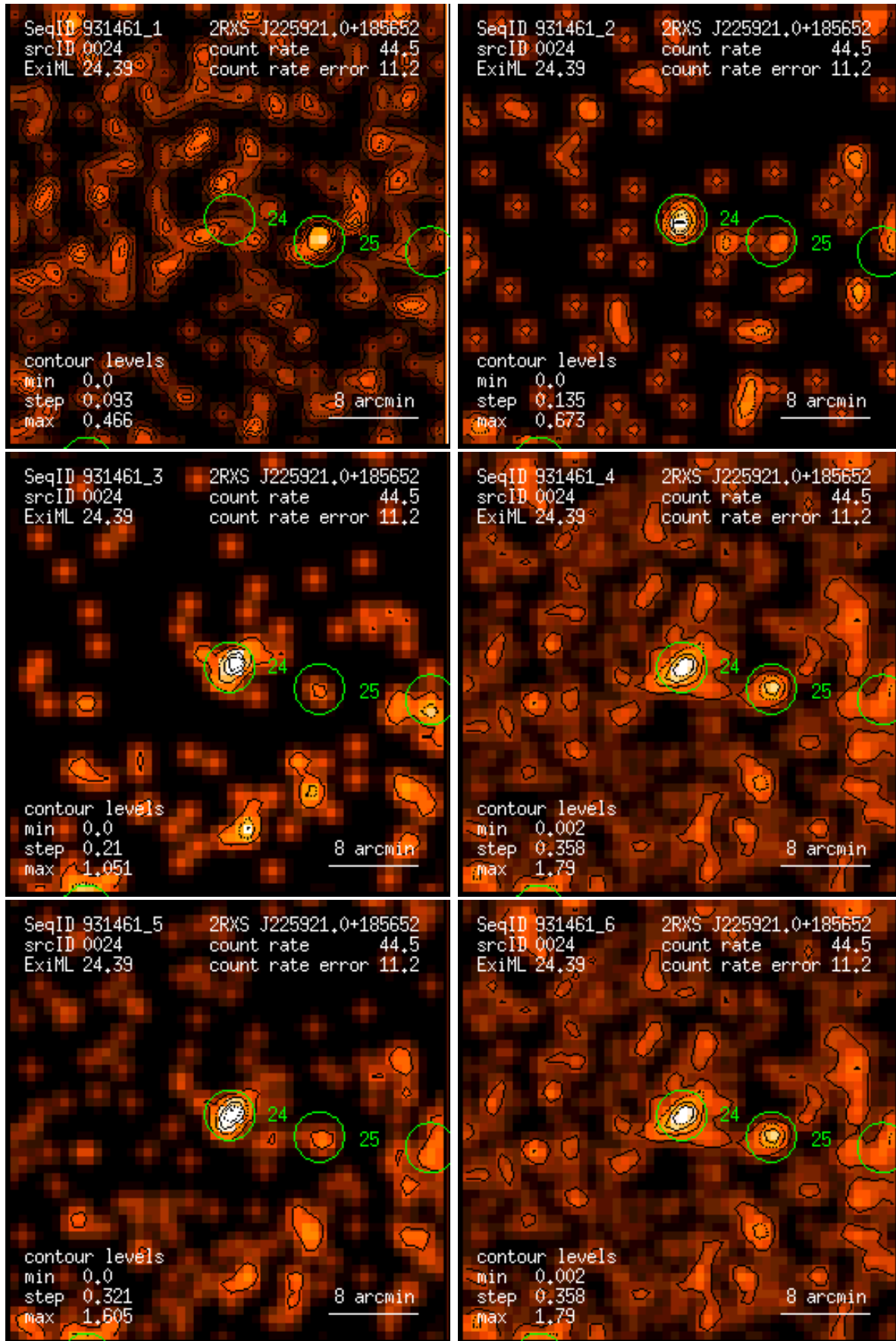
Figure 24: RASS 931461: detection 0024: band rate images, Gaussian filter: (1) PSPC channels 11 – 41, (2) 52 – 90, (3) 91 – 201, (4) 11 – 235, (5) 52 – 201, (6) 11 – 201. Broad band rates in counts/ks. Band rate contour levels in counts/ks/arcmin 2 .
