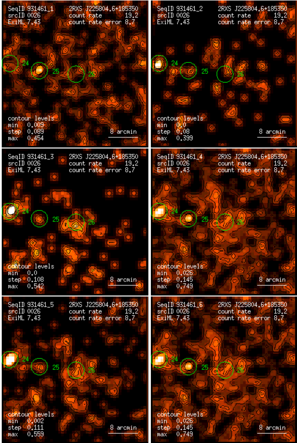
Figure 26: RASS 931461: detection 0026: band rate images, Gaussian filter: (1) PSPC channels 11 – 41, (2) 52 – 90, (3) 91 – 201, (4) 11 – 235, (5) 52 – 201, (6) 11 – 201. Broad band rates in counts/ks. Band rate contour levels in counts/ks/arcmin 2 .
