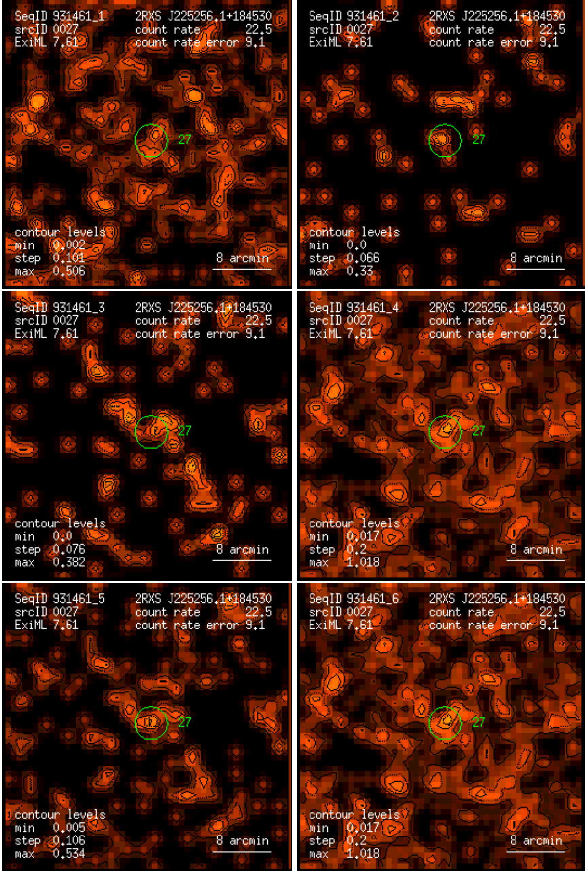
Figure 27: RASS 931461: detection 0027: band rate images, Gaussian filter: (1) PSPC channels 11 – 41, (2) 52 – 90, (3) 91 – 201, (4) 11 – 235, (5) 52 – 201, (6) 11 – 201. Broad band rates in counts/ks. Band rate contour levels in counts/ks/arcmin 2 .
