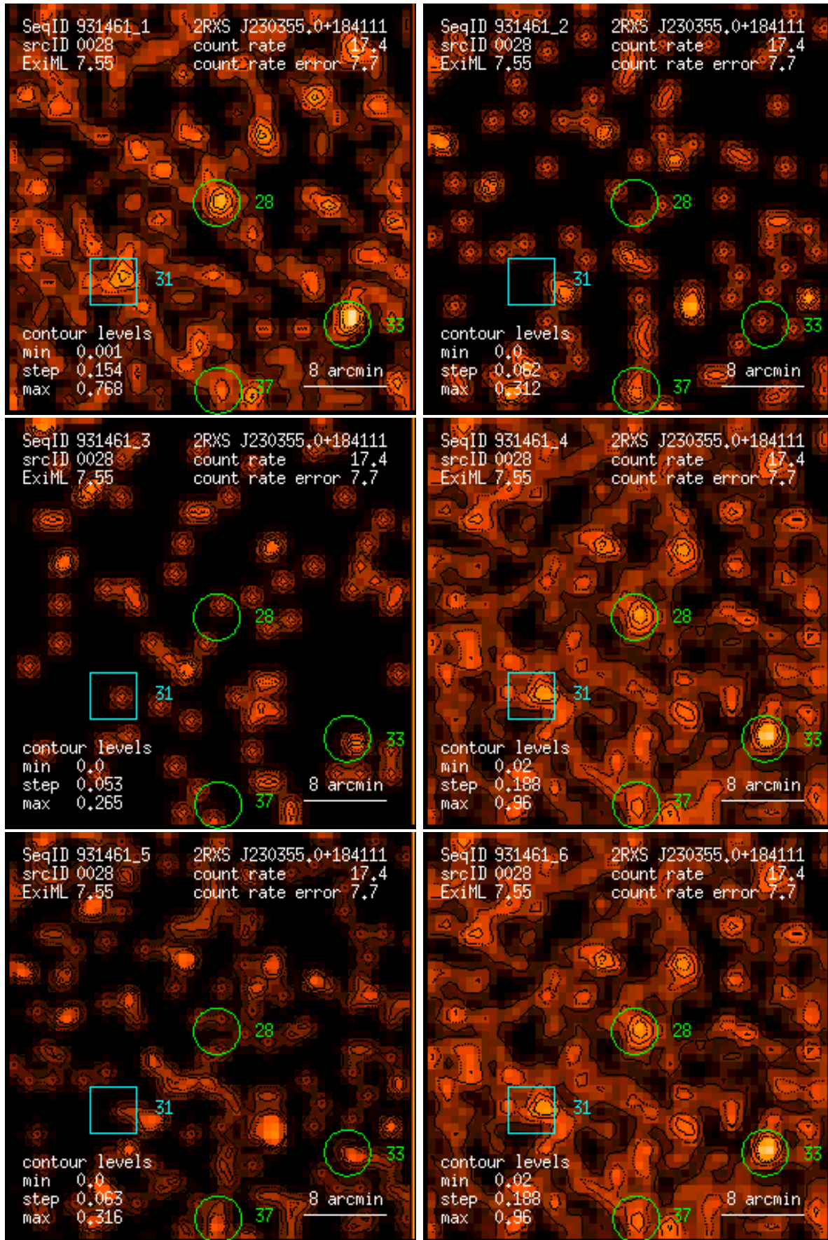
Figure 28: RASS 931461: detection 0028: band rate images, Gaussian filter: (1) PSPC channels 11 – 41, (2) 52 – 90, (3) 91 – 201, (4) 11 – 235, (5) 52 – 201, (6) 11 – 201. Broad band rates in counts/ks. Band rate contour levels in counts/ks/arcmin 2 .
