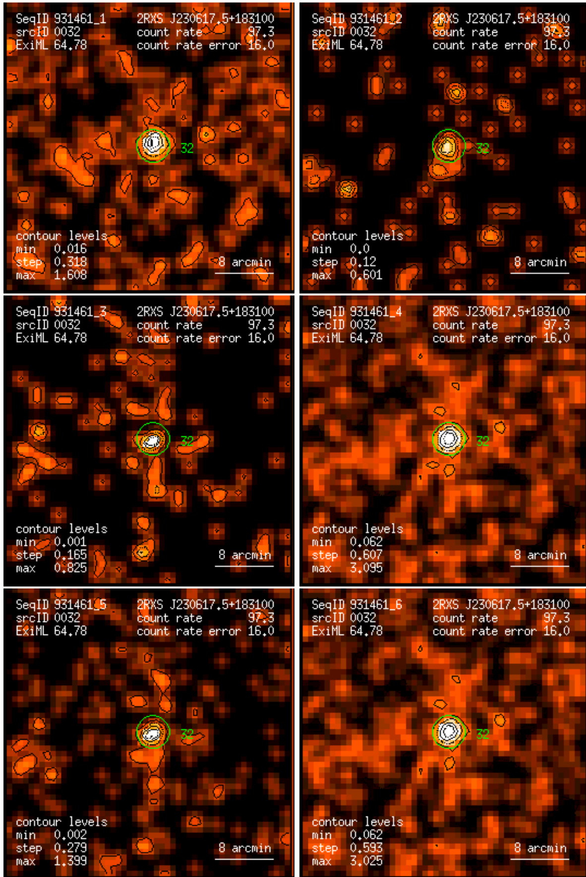
Figure 32: RASS 931461: detection 0032: band rate images, Gaussian filter: (1) PSPC channels 11 – 41, (2) 52 – 90, (3) 91 – 201, (4) 11 – 235, (5) 52 – 201, (6) 11 – 201. Broad band rates in counts/ks. Band rate contour levels in counts/ks/arcmin 2 .
