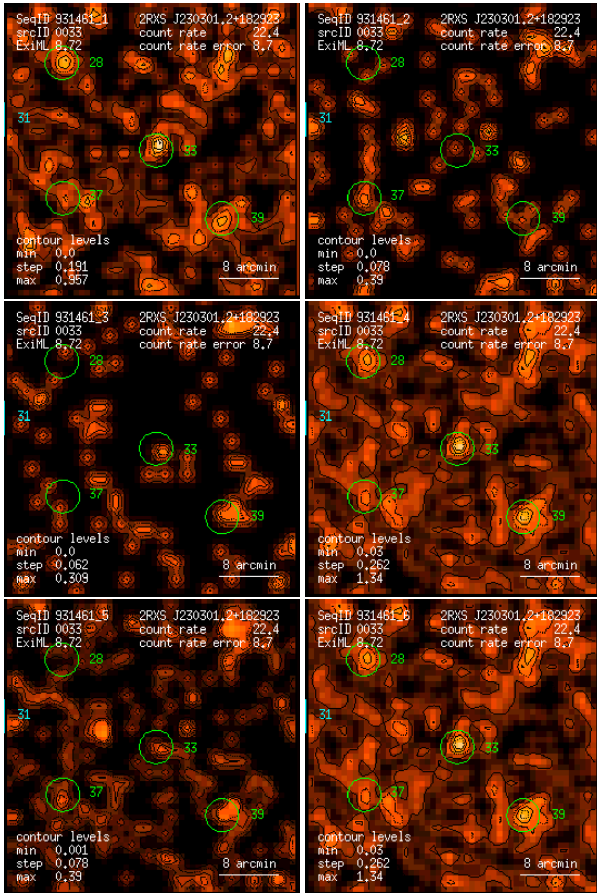
Figure 33: RASS 931461: detection 0033: band rate images, Gaussian filter: (1) PSPC channels 11 – 41, (2) 52 – 90, (3) 91 – 201, (4) 11 – 235, (5) 52 – 201, (6) 11 – 201. Broad band rates in counts/ks. Band rate contour levels in counts/ks/arcmin 2 .
