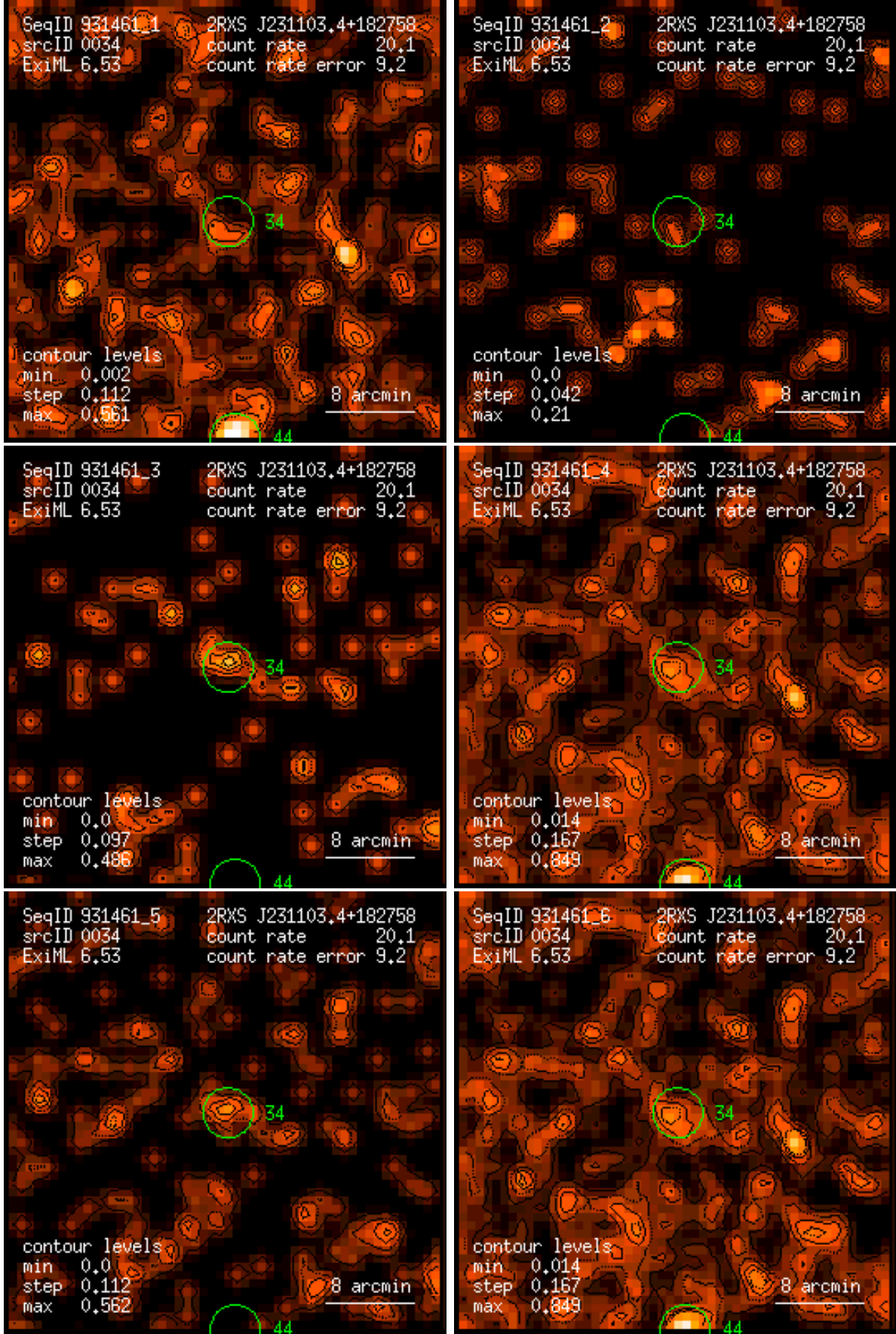
Figure 34: RASS 931461: detection 0034: band rate images, Gaussian filter: (1) PSPC channels 11 – 41, (2) 52 – 90, (3) 91 – 201, (4) 11 – 235, (5) 52 – 201, (6) 11 – 201. Broad band rates in counts/ks. Band rate contour levels in counts/ks/arcmin 2 .
