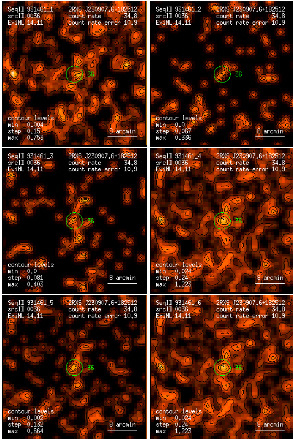
Figure 36: RASS 931461: detection 0036: band rate images, Gaussian filter: (1) PSPC channels 11 – 41, (2) 52 – 90, (3) 91 – 201, (4) 11 – 235, (5) 52 – 201, (6) 11 – 201. Broad band rates in counts/ks. Band rate contour levels in counts/ks/arcmin 2 .
