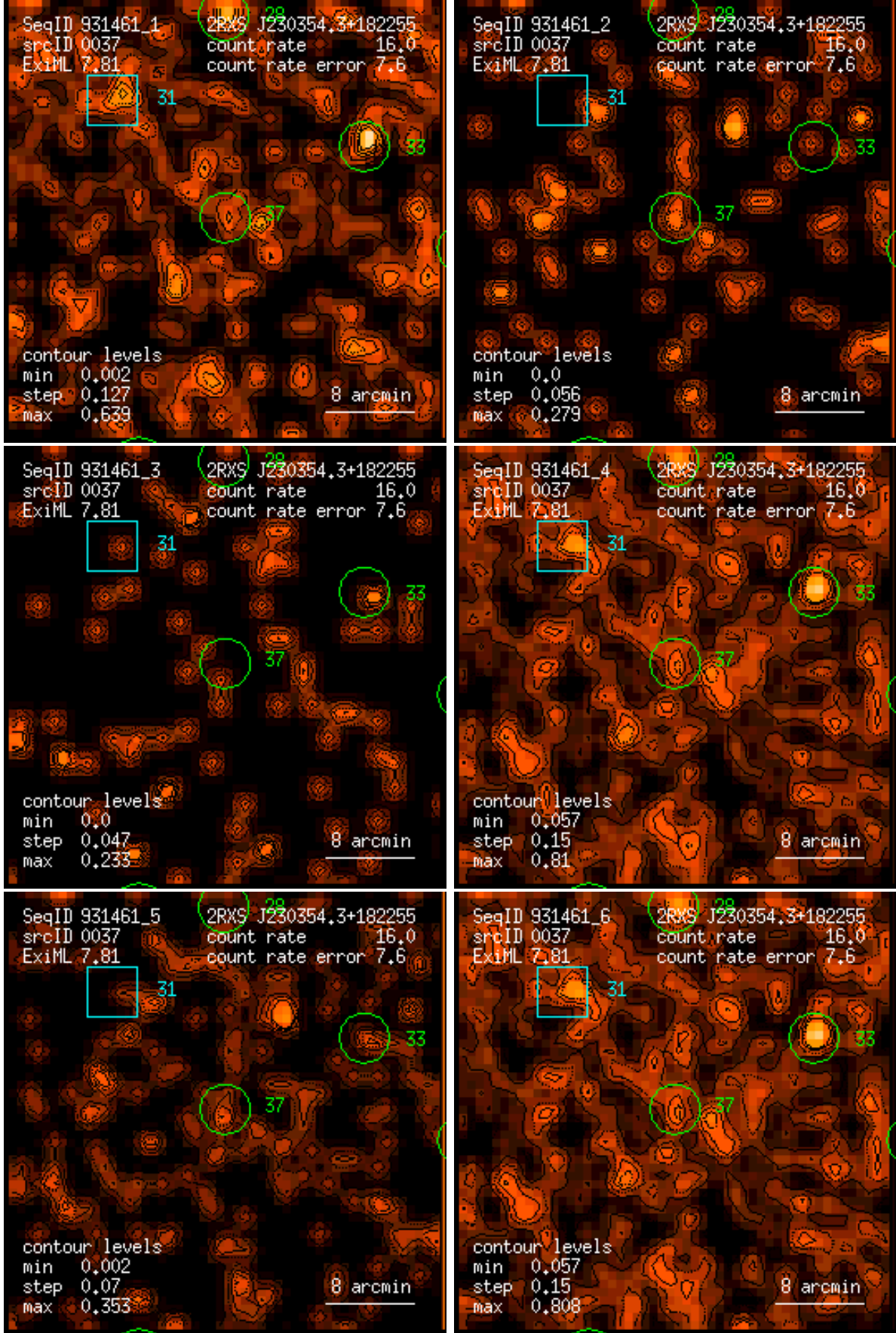
Figure 37: RASS 931461: detection 0037: band rate images, Gaussian filter: (1) PSPC channels 11 – 41, (2) 52 – 90, (3) 91 – 201, (4) 11 – 235, (5) 52 – 201, (6) 11 – 201. Broad band rates in counts/ks. Band rate contour levels in counts/ks/arcmin 2 .
