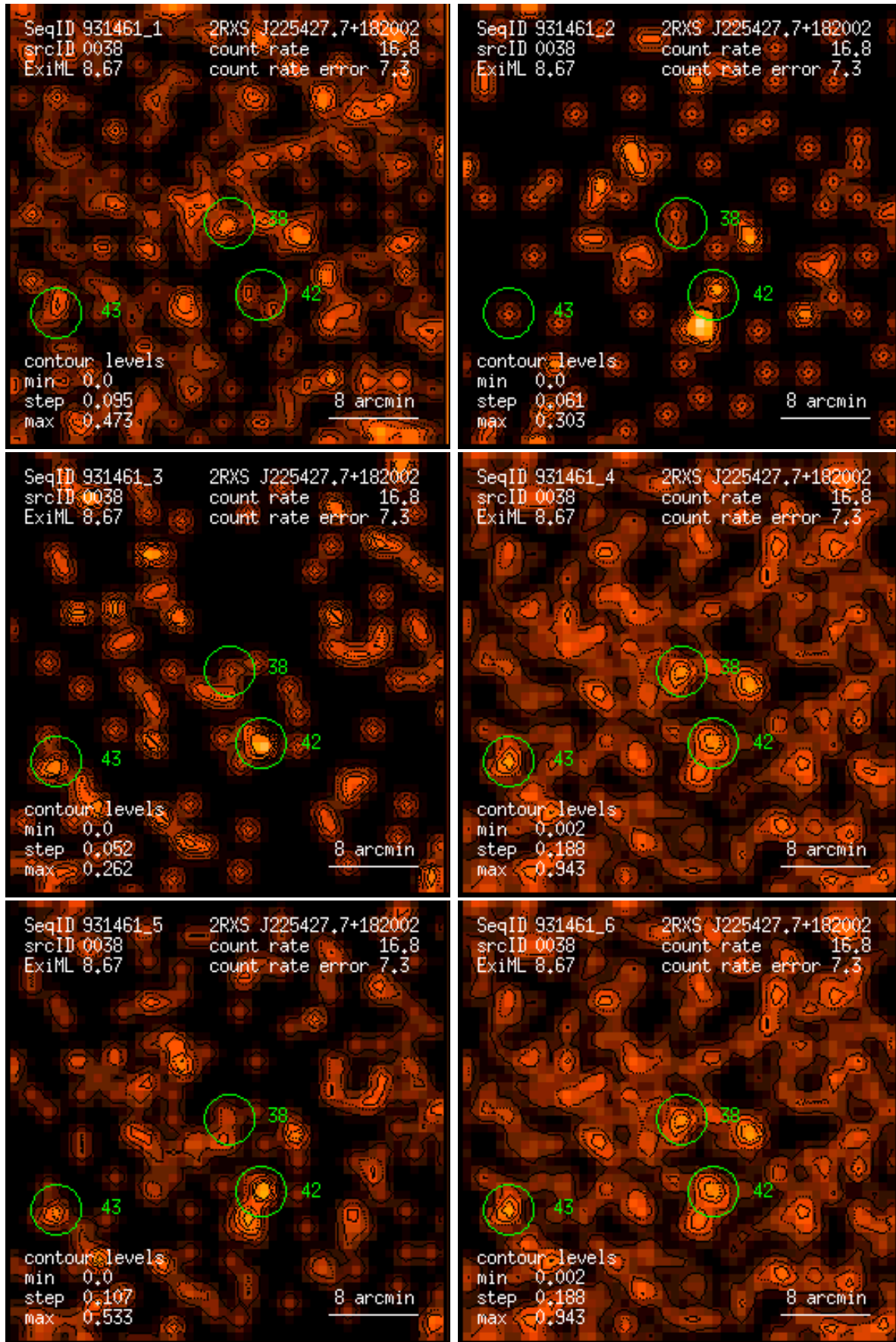
Figure 38: RASS 931461: detection 0038: band rate images, Gaussian filter: (1) PSPC channels 11 – 41, (2) 52 – 90, (3) 91 – 201, (4) 11 – 235, (5) 52 – 201, (6) 11 – 201. Broad band rates in counts/ks. Band rate contour levels in counts/ks/arcmin 2 .
