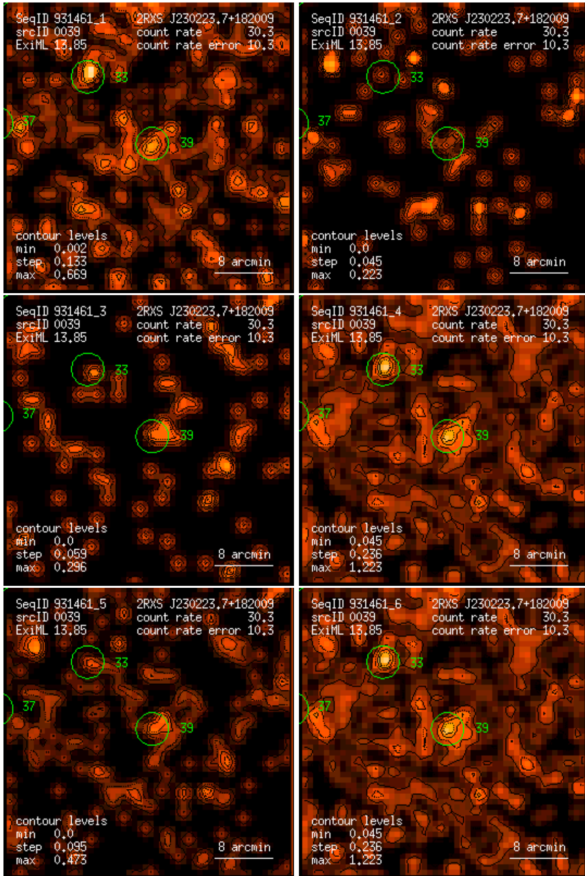
Figure 39: RASS 931461: detection 0039: band rate images, Gaussian filter: (1) PSPC channels 11 – 41, (2) 52 – 90, (3) 91 – 201, (4) 11 – 235, (5) 52 – 201, (6) 11 – 201. Broad band rates in counts/ks. Band rate contour levels in counts/ks/arcmin 2 .
