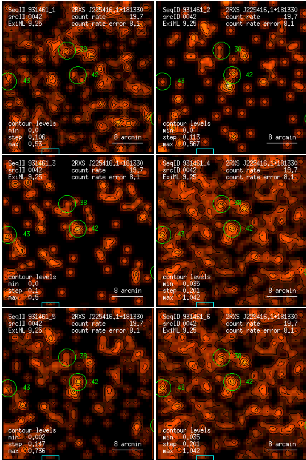
Figure 42: RASS 931461: detection 0042: band rate images, Gaussian filter: (1) PSPC channels 11 – 41, (2) 52 – 90, (3) 91 – 201, (4) 11 – 235, (5) 52 – 201, (6) 11 – 201. Broad band rates in counts/ks. Band rate contour levels in counts/ks/arcmin 2 .
