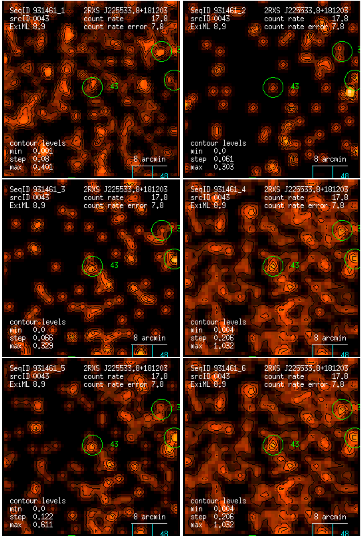
Figure 43: RASS 931461: detection 0043: band rate images, Gaussian filter: (1) PSPC channels 11 – 41, (2) 52 – 90, (3) 91 – 201, (4) 11 – 235, (5) 52 – 201, (6) 11 – 201. Broad band rates in counts/ks. Band rate contour levels in counts/ks/arcmin 2 .
