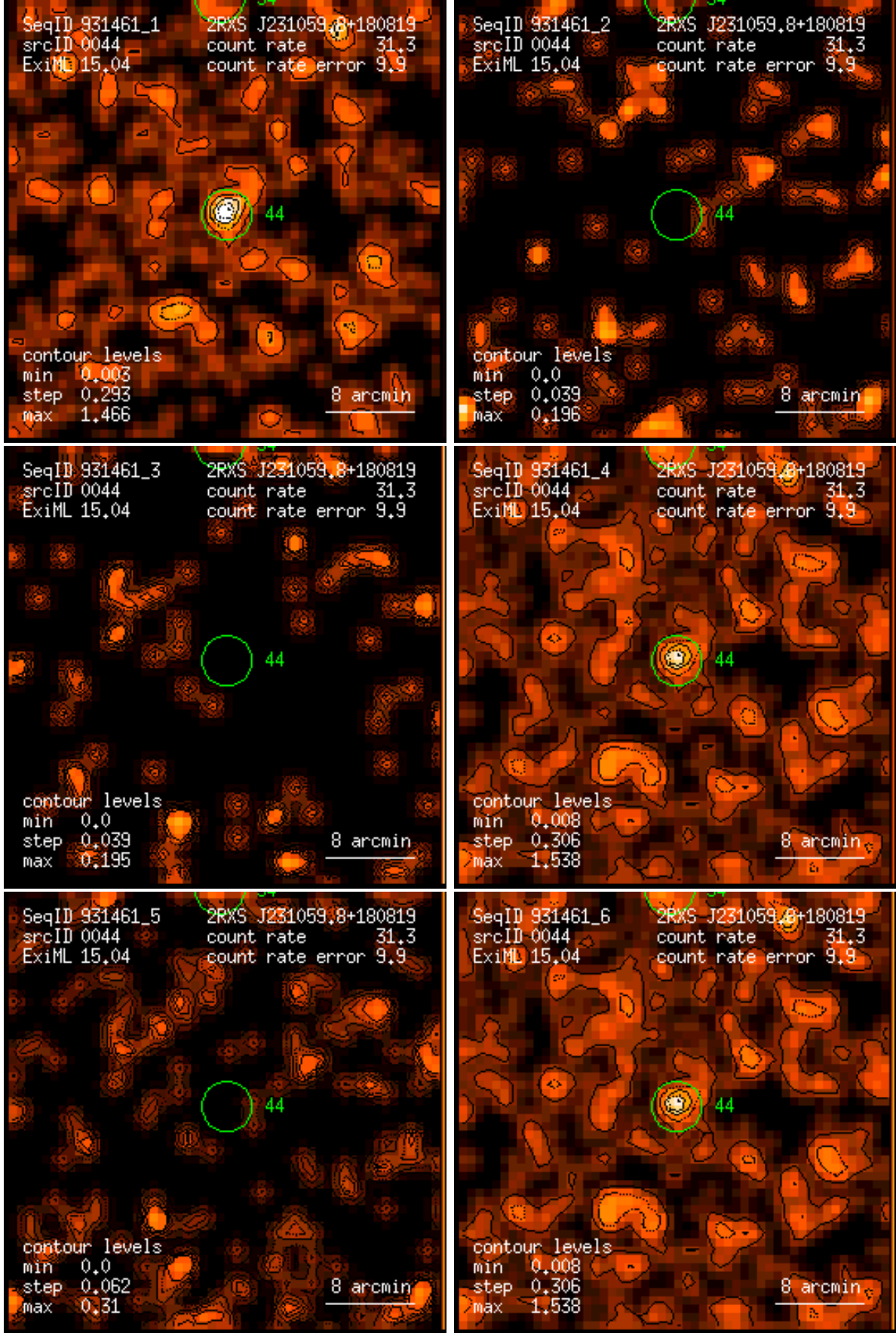
Figure 44: RASS 931461: detection 0044: band rate images, Gaussian filter: (1) PSPC channels 11 – 41, (2) 52 – 90, (3) 91 – 201, (4) 11 – 235, (5) 52 – 201, (6) 11 – 201. Broad band rates in counts/ks. Band rate contour levels in counts/ks/arcmin 2 .
