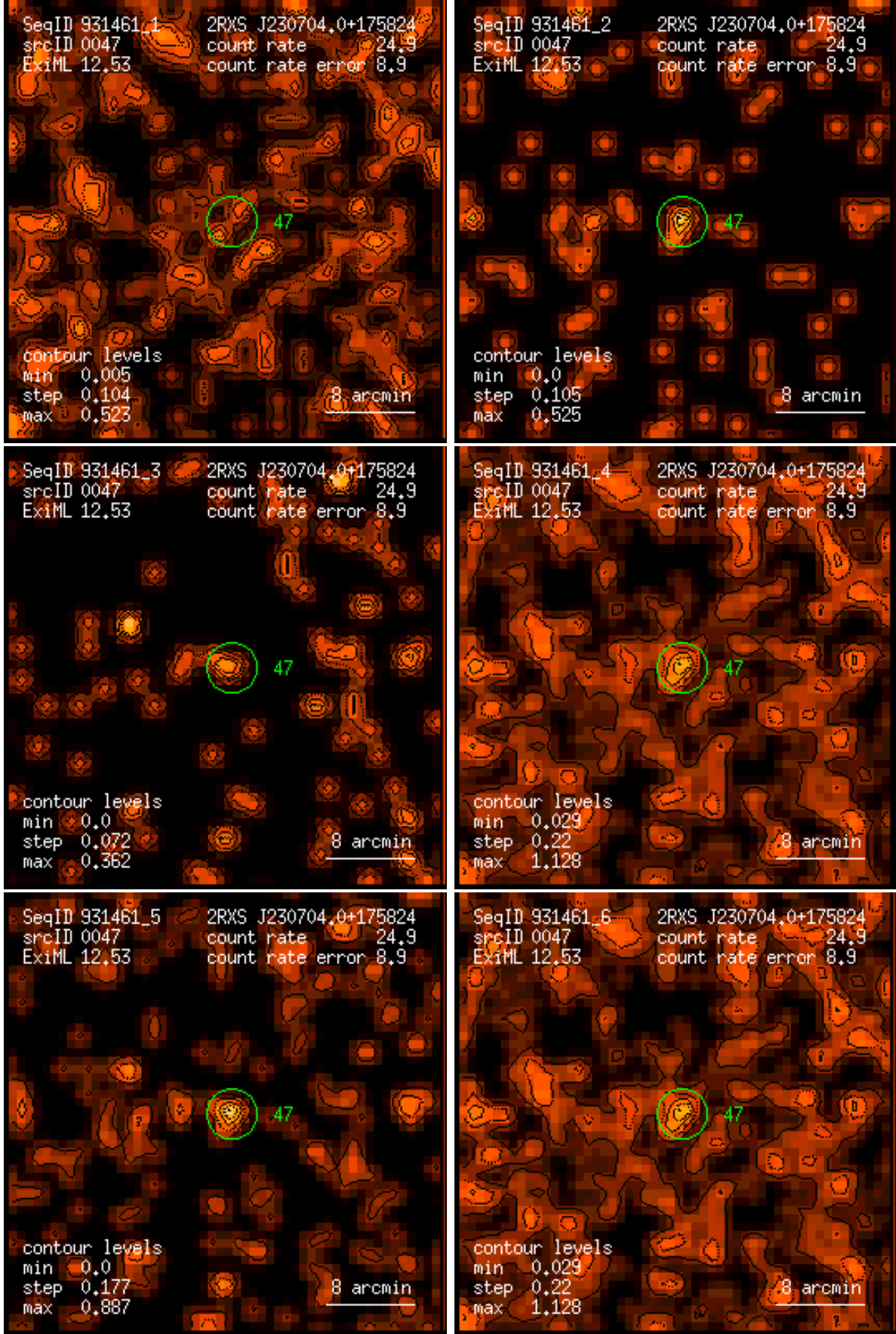
Figure 47: RASS 931461: detection 0047: band rate images, Gaussian filter: (1) PSPC channels 11 – 41, (2) 52 – 90, (3) 91 – 201, (4) 11 – 235, (5) 52 – 201, (6) 11 – 201. Broad band rates in counts/ks. Band rate contour levels in counts/ks/arcmin 2 .
