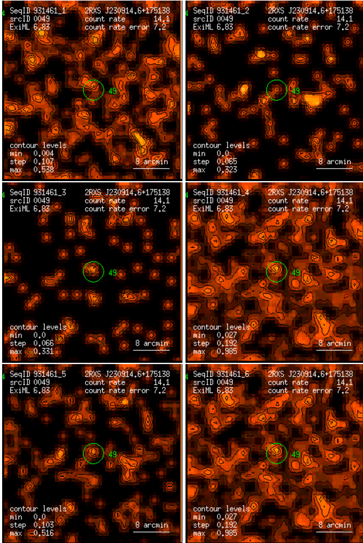
Figure 49: RASS 931461: detection 0049: band rate images, Gaussian filter: (1) PSPC channels 11 – 41, (2) 52 – 90, (3) 91 – 201, (4) 11 – 235, (5) 52 – 201, (6) 11 – 201. Broad band rates in counts/ks. Band rate contour levels in counts/ks/arcmin 2 .
