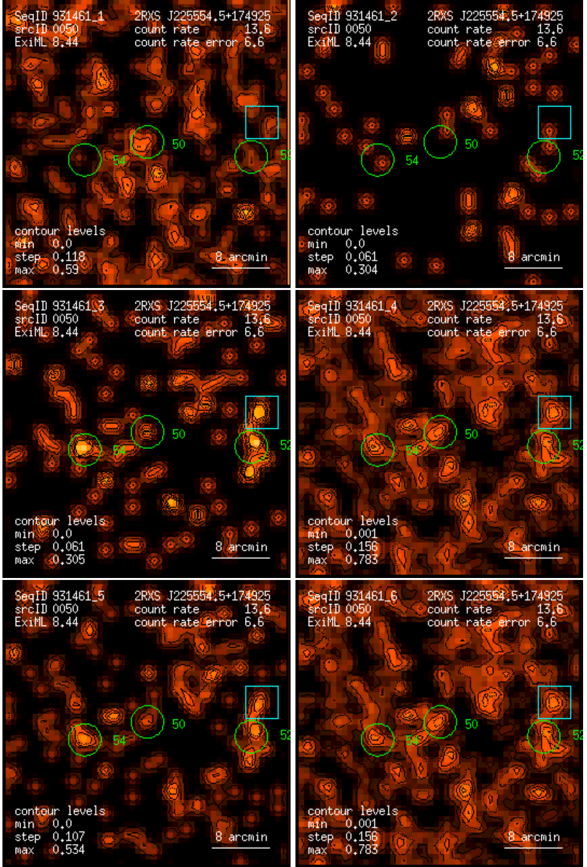
Figure 50: RASS 931461: detection 0050: band rate images, Gaussian filter: (1) PSPC channels 11 – 41, (2) 52 – 90, (3) 91 – 201, (4) 11 – 235, (5) 52 – 201, (6) 11 – 201. Broad band rates in counts/ks. Band rate contour levels in counts/ks/arcmin 2 .
