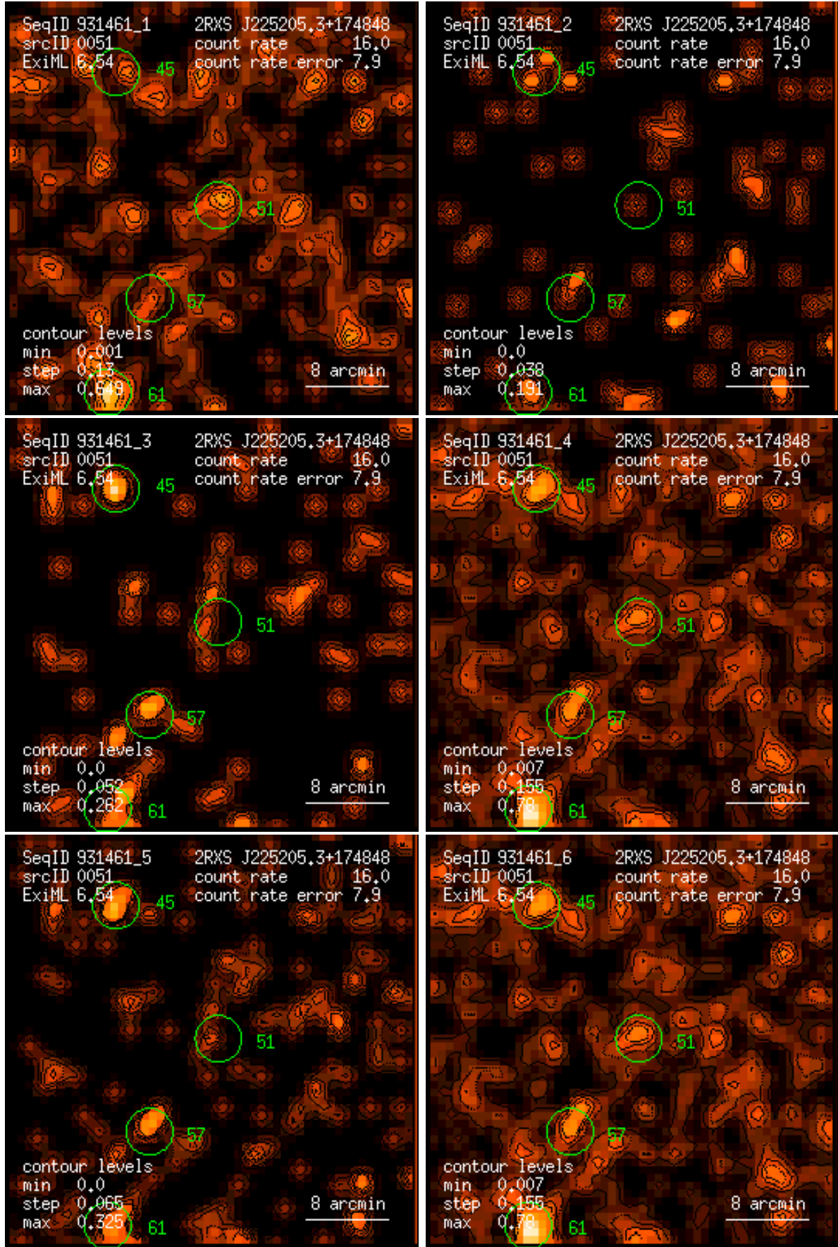
Figure 51: RASS 931461: detection 0051: band rate images, Gaussian filter: (1) PSPC channels 11 – 41, (2) 52 – 90, (3) 91 – 201, (4) 11 – 235, (5) 52 – 201, (6) 11 – 201. Broad band rates in counts/ks. Band rate contour levels in counts/ks/arcmin 2 .
