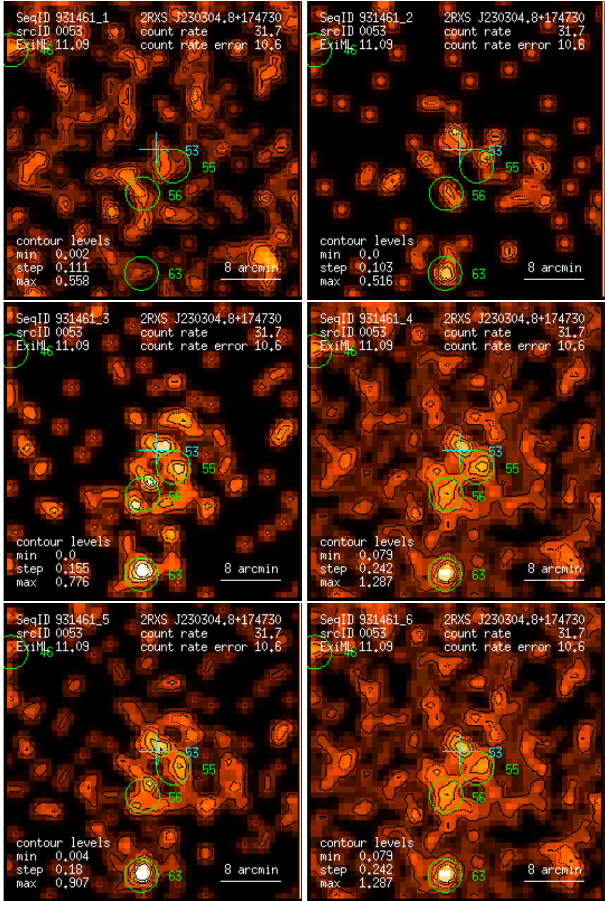
Figure 53: RASS 931461: detection 0053: band rate images, Gaussian filter: (1) PSPC channels 11 – 41, (2) 52 – 90, (3) 91 – 201, (4) 11 – 235, (5) 52 – 201, (6) 11 – 201. Broad band rates in counts/ks. Band rate contour levels in counts/ks/arcmin 2 .
