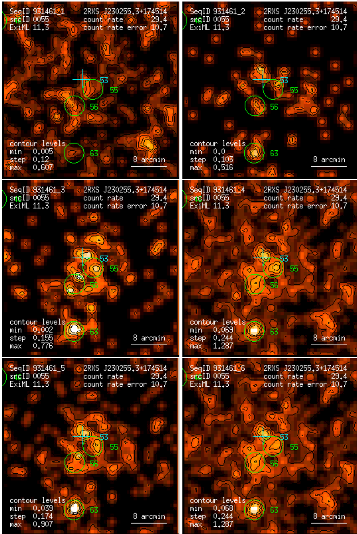
Figure 55: RASS 931461: detection 0055: band rate images, Gaussian filter: (1) PSPC channels 11 – 41, (2) 52 – 90, (3) 91 – 201, (4) 11 – 235, (5) 52 – 201, (6) 11 – 201. Broad band rates in counts/ks. Band rate contour levels in counts/ks/arcmin 2 .
