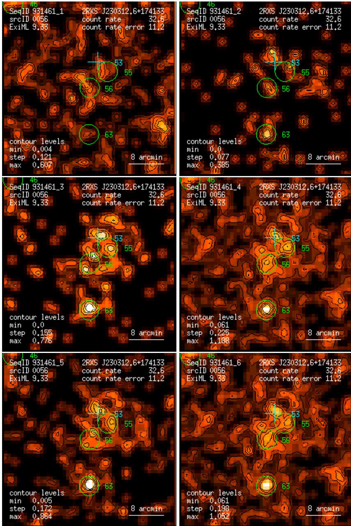
Figure 56: RASS 931461: detection 0056: band rate images, Gaussian filter: (1) PSPC channels 11 – 41, (2) 52 – 90, (3) 91 – 201, (4) 11 – 235, (5) 52 – 201, (6) 11 – 201. Broad band rates in counts/ks. Band rate contour levels in counts/ks/arcmin 2 .
